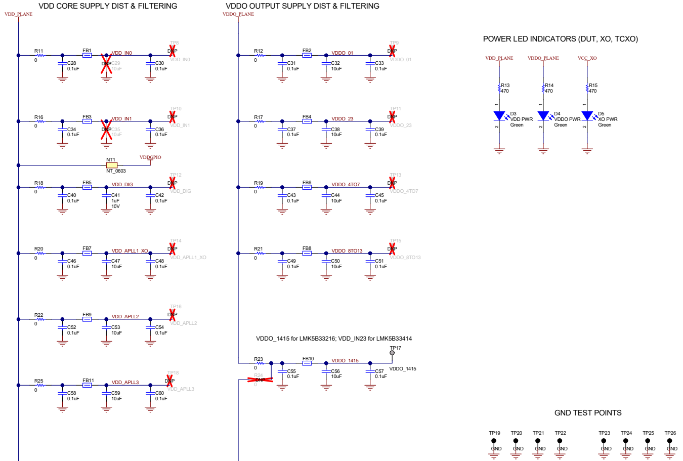
Figure 4-3. Power Distribution
