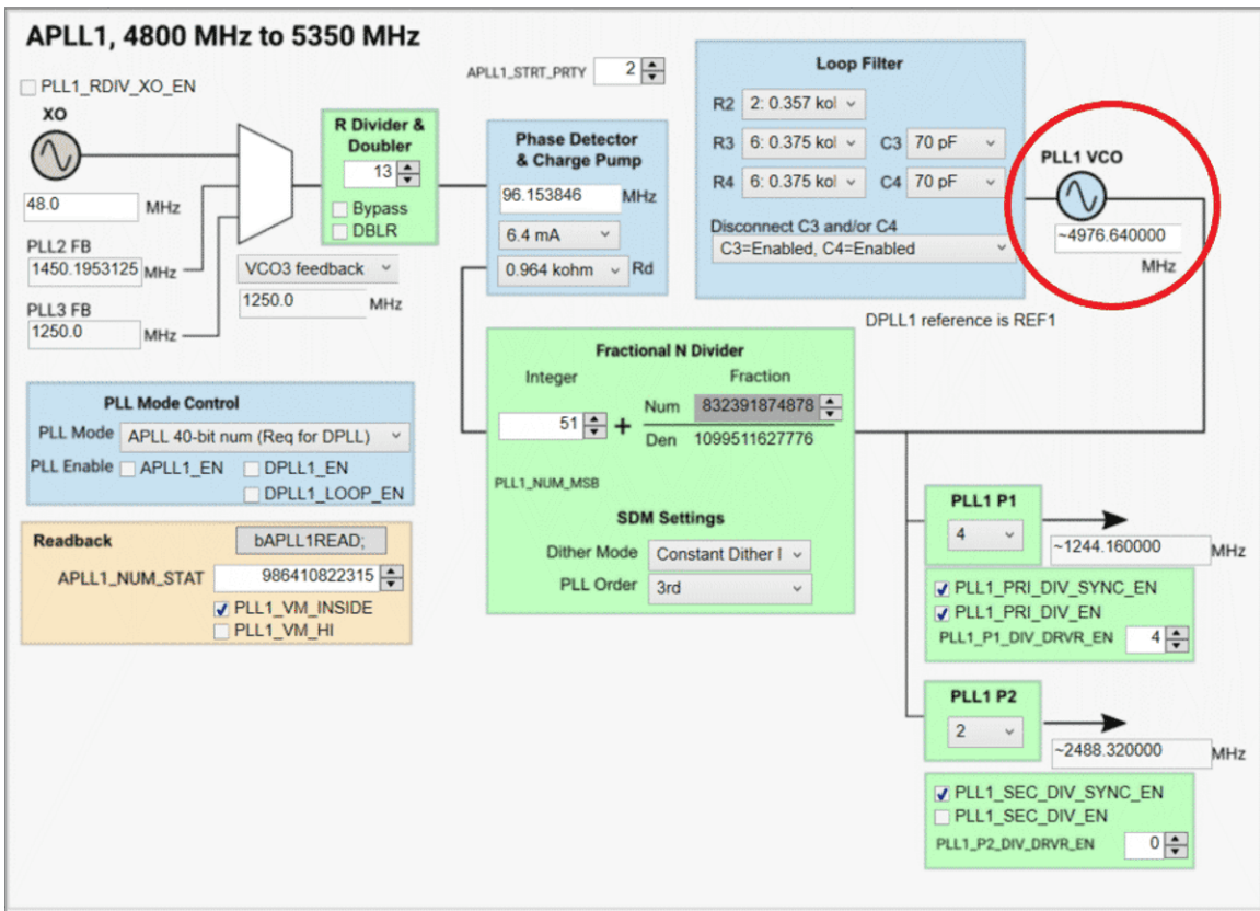
Figure 6-13. APLL1 Page
