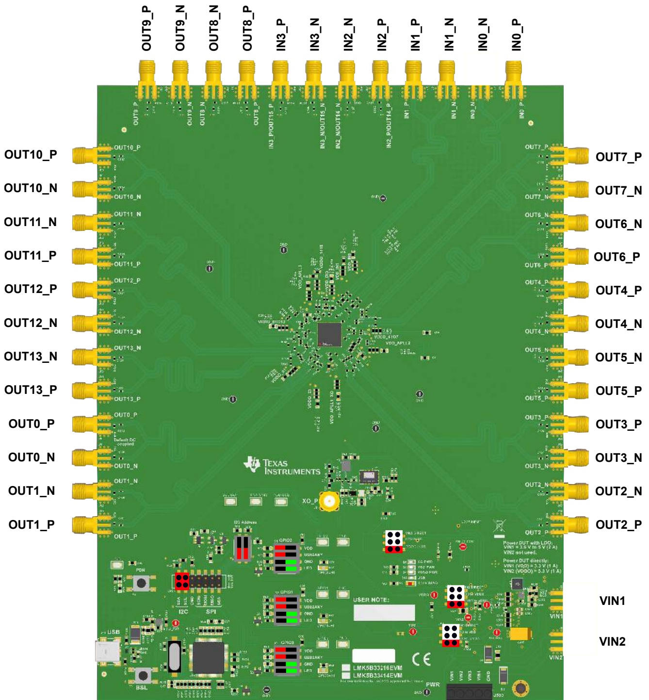
Figure 1-1. LMK5B33414EVM Default Setting of Jumpers and DIP Switches
