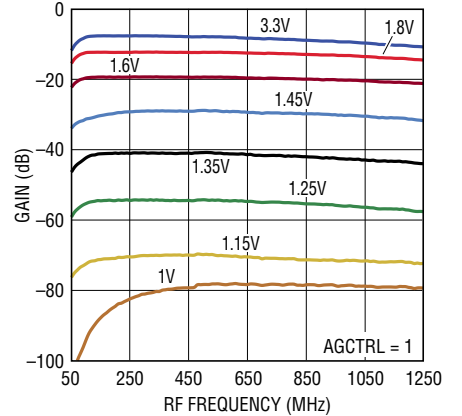
Gain vs RF Frequency and V_{CTRL}
