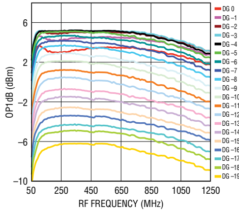
Output 1dB Compression Point vs RF Frequency and Digital Gain Setting at -10°C
