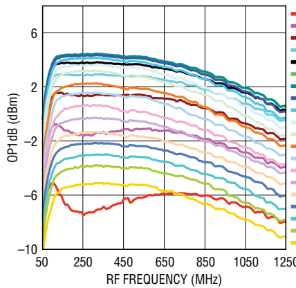
Output 1dB Compression Point vs RF Frequency and Digital Gain Setting at 105°C
