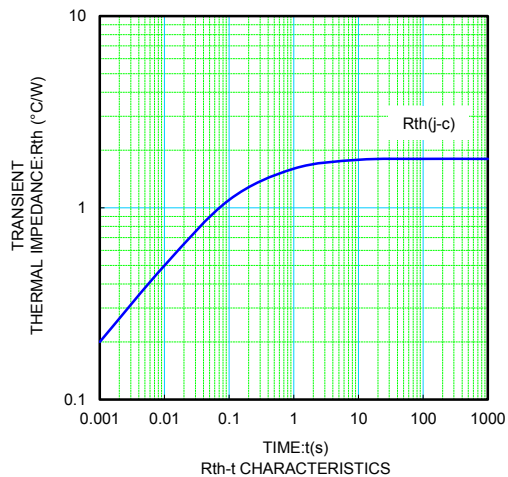
R_{th(j-c)} CHARACTERISTICS
