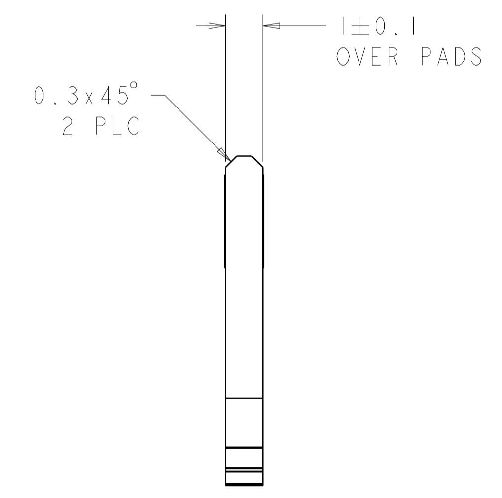
RECOMMENDED MATING PCB CONFIGURATION
