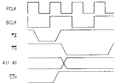
Figure 11-5. MC68040 Address Hold Time
