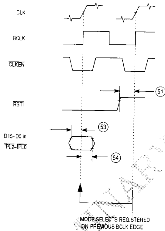
Figure 12-14. Reset Configuration Timing
