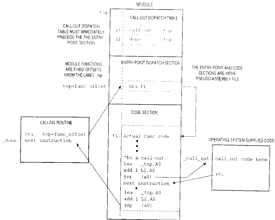
Figure C-3. Module Call-In, Call-Out Example
