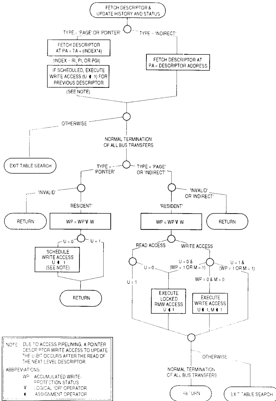
Figure 4-9. Detailed Flowchart of Descriptor Fetch Operation
