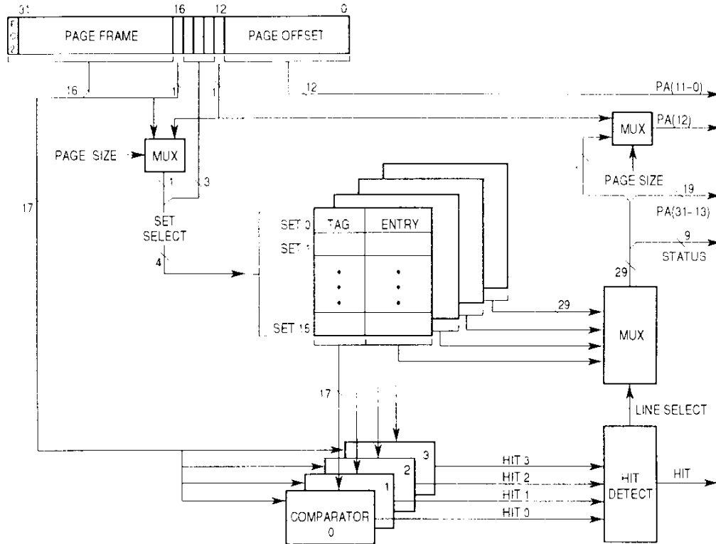
Figure 4-19. ATC Organization
