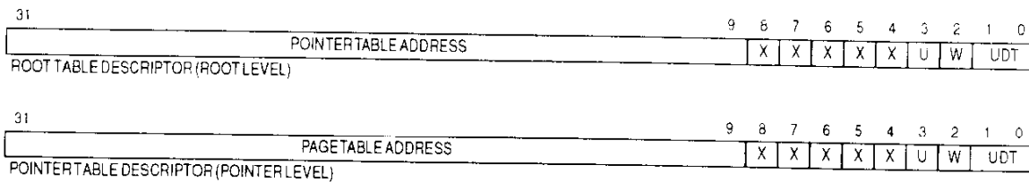
Figure 4-10. Table Descriptor Formats
