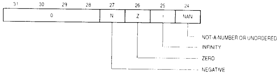
Figure 6-4. Floating-Point Condition Code (FPSR)
