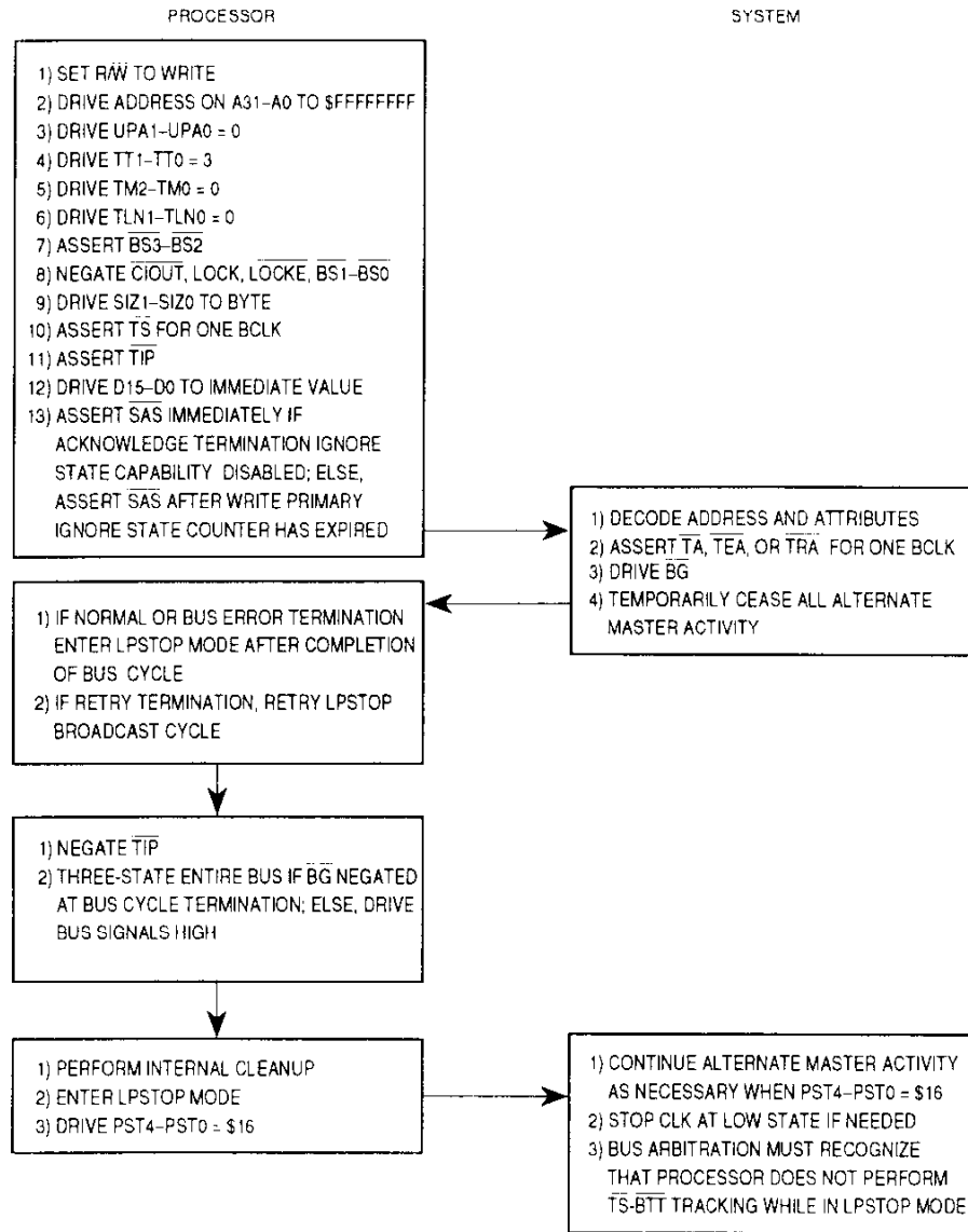
Figure 7-32. LPSTOP Broadcast Cycle Flowchart
