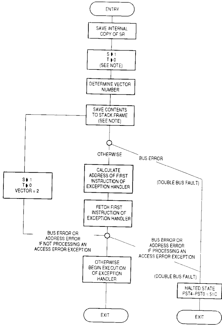
Figure 8-1. General Exception Processing Flowchart
