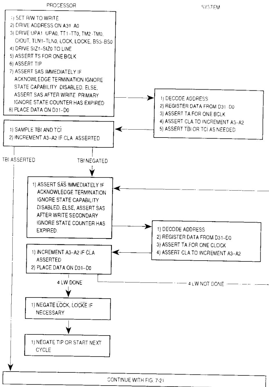
Figure 7-20. Line Write Cycle Flowchart
