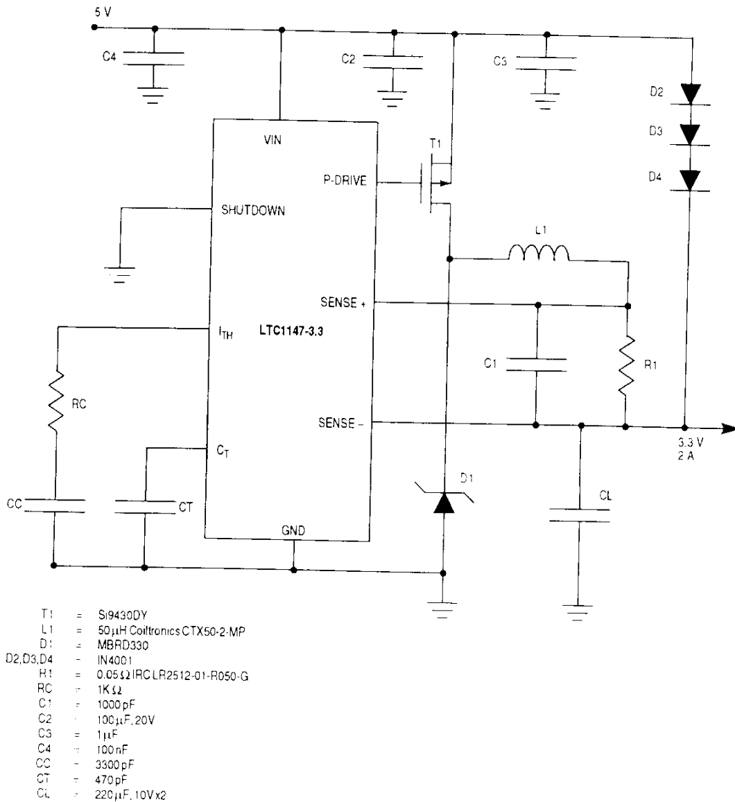
Figure 11-2. LTC1147 Voltage Regulator Solution
