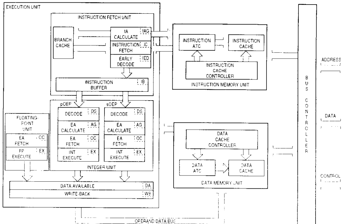
Figure 1-1. MC68060 Block Diagram
