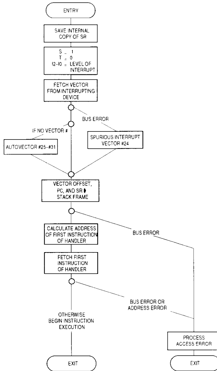
Figure 8-4. Interrupt Exception Processing Flowchart
