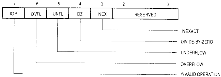
Figure 6-7. Floating-Point Accrued Exception Byte (FPSR)
