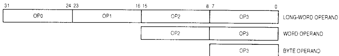
Figure 7-6. Internal Operand Representation
