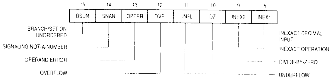
Figure 6-6. Floating-Point Exception Status Byte (FPSR)
