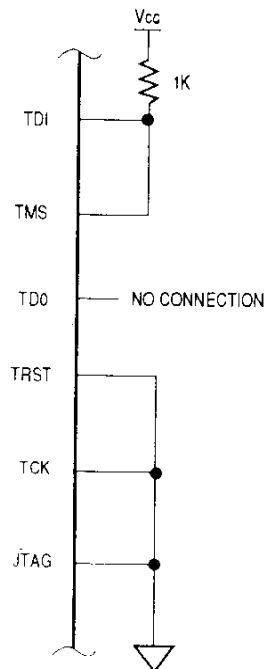
Figure 9-9. Circuit Disabling IEEE Standard 1149.1
