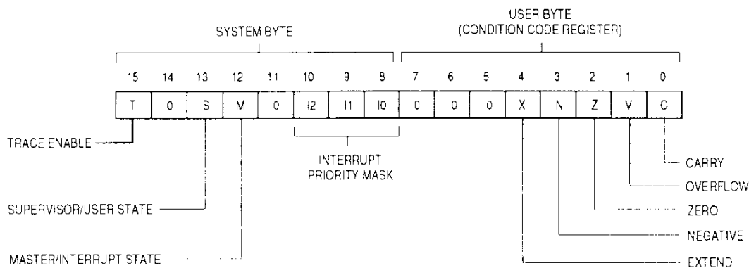
Figure 3-4. Status Register
