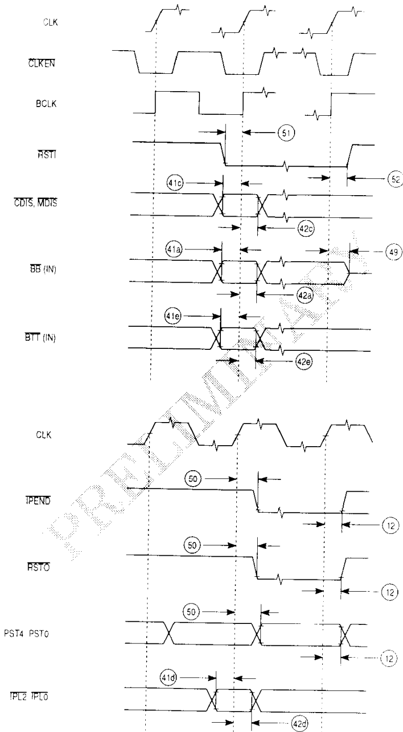
Figure 12-20. Other Signals Timing
