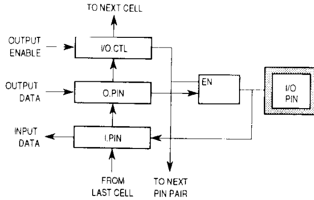
Figure 9-7. General Arrangement of Bidirectional Pin Cells
