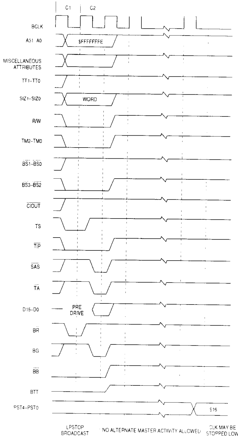
Figure 7-34. LPSTOP Broadcast Bus Cycle Timing, \overline{BG} Asserted
