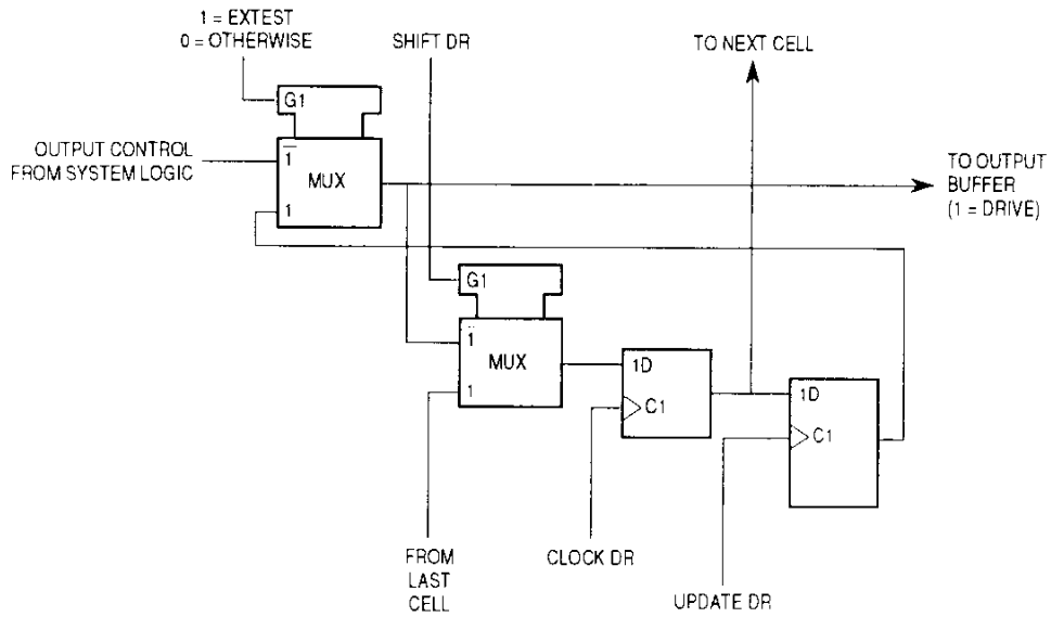
Figure 9-6. Output Control Cell (IO.CtI)
