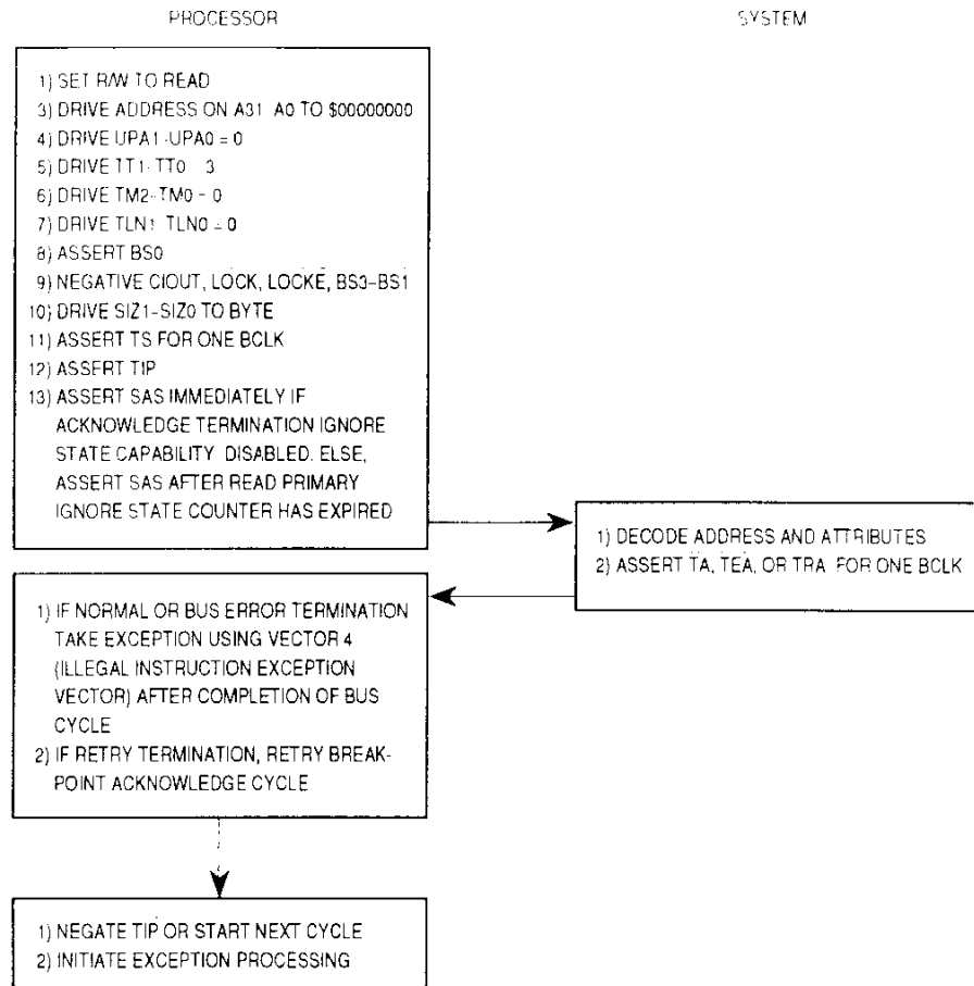
Figure 7-30. Breakpoint Interrupt Acknowledge Cycle Flowchart
