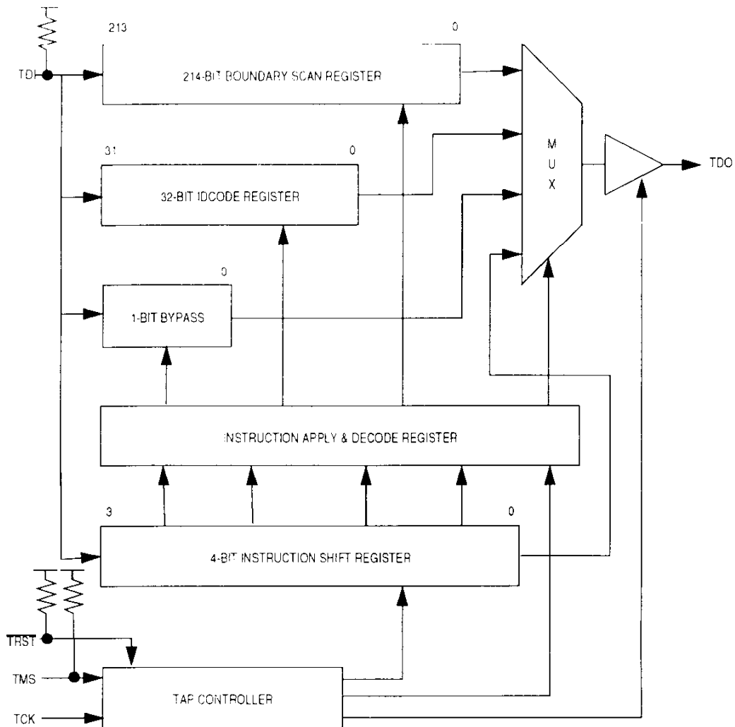
Figure 9-1. JTAG Test Logic Block Diagram
