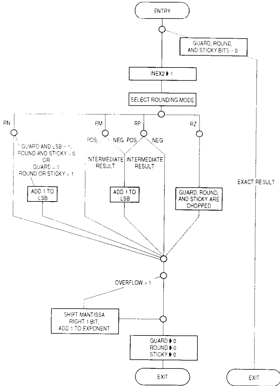
Figure 6-9. Rounding Algorithm Flowchart
