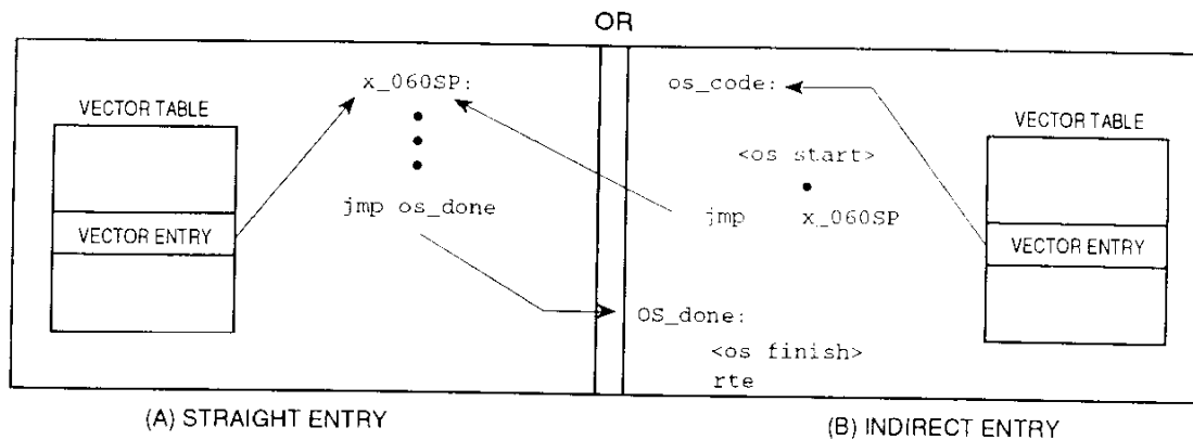
Figure C-12. Vector Table and M68060SP Relationship
