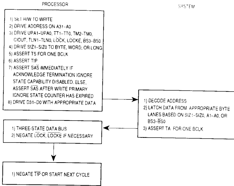
Figure 7-18. Byte, Word, and Long-Word Write Transfer Flowchart
