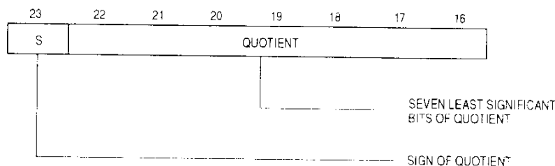
Figure 6-5. Floating-Point Quotient Byte (FPSR)
