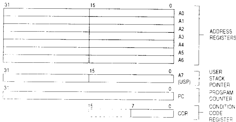
Figure 3-2. Integer Unit User Programming Model
