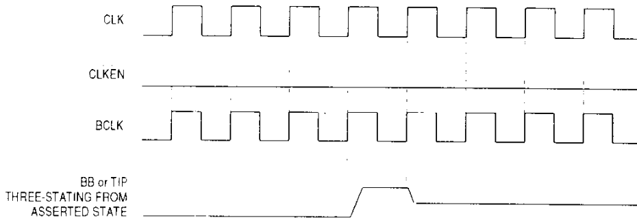
Figure 7-2. Full-Speed Clock
