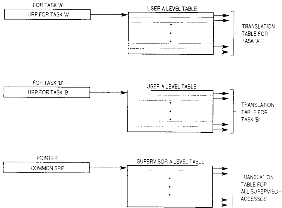
Figure 4-16. Translation Table Structure for Two Tasks
