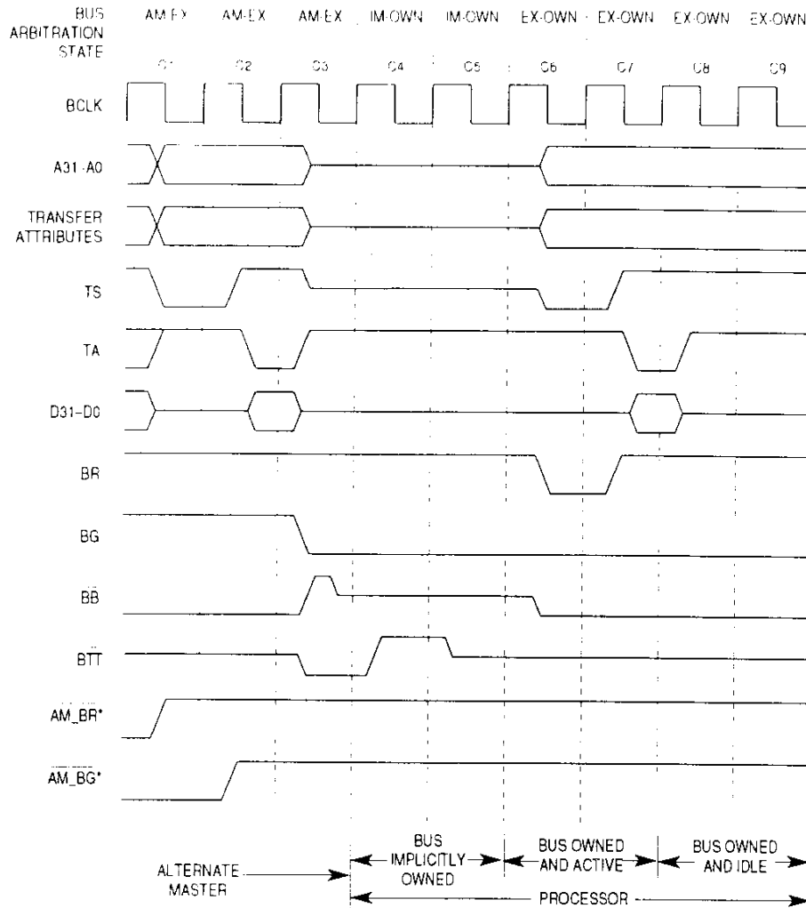
Figure 7-45. Implicit Bus Ownership Arbitration Timing
