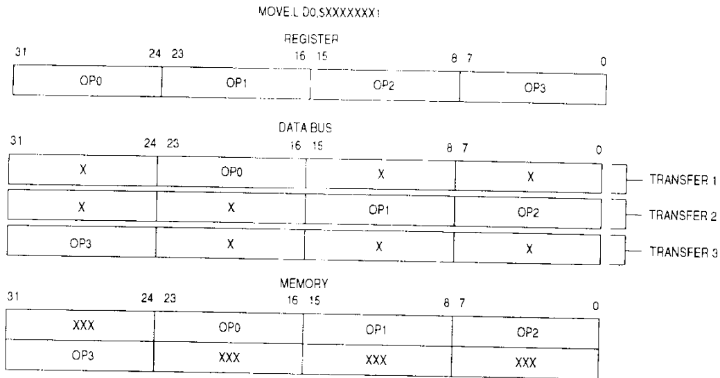
Figure 7-9. Example of a Misaligned Long-Word Transfer
