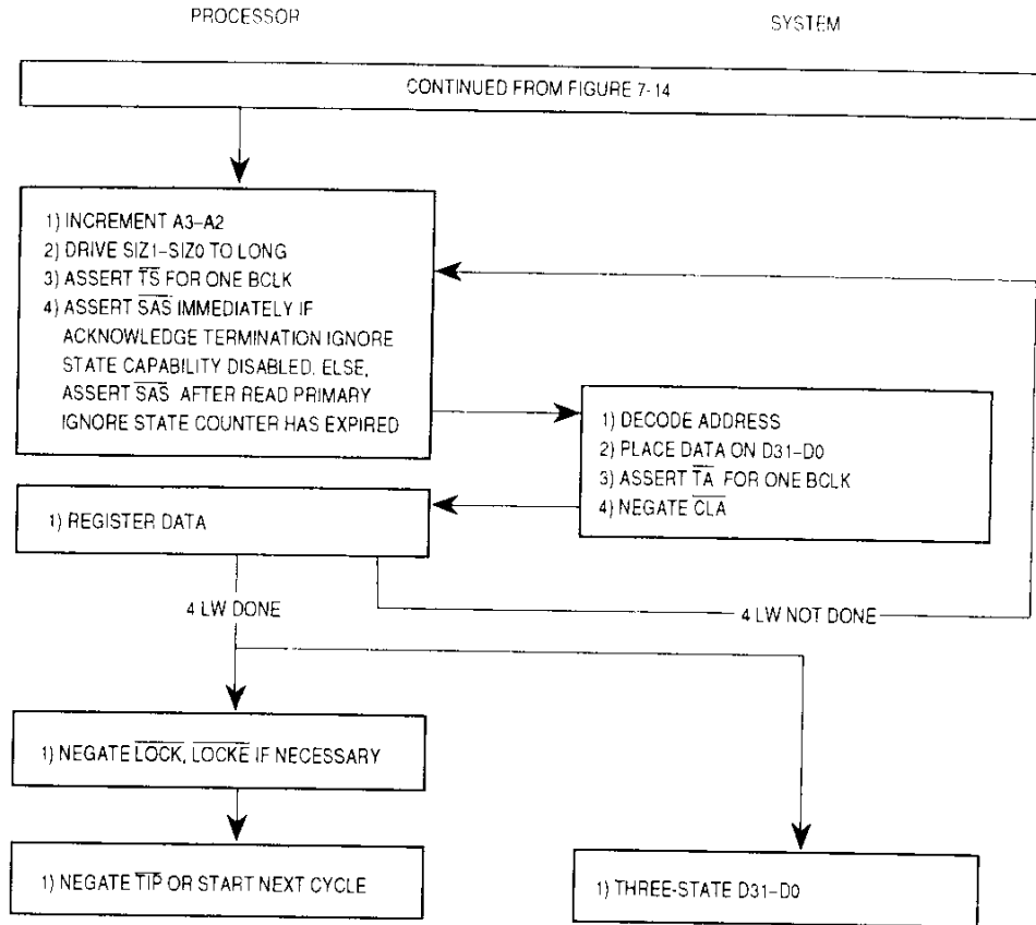
Figure 7-16. Burst-Inhibited Line Read Cycle Flowchart
