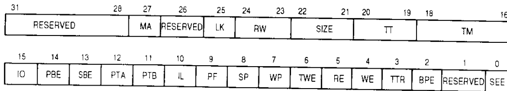
Figure 8-6. Fault Status Long-Word Format
