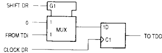
Figure 9-8. JTAG Bypass Register
