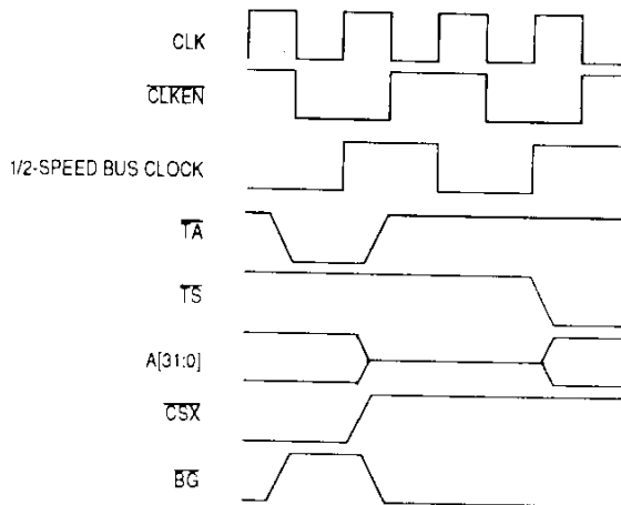
Figure 11-7. MC68060 Address Hold Time Fix
