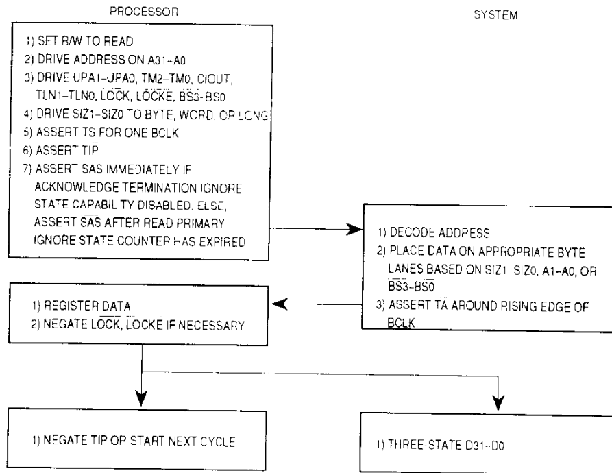
Figure 7-12. Byte, Word, and Long-Word Read Cycle Flowchart
