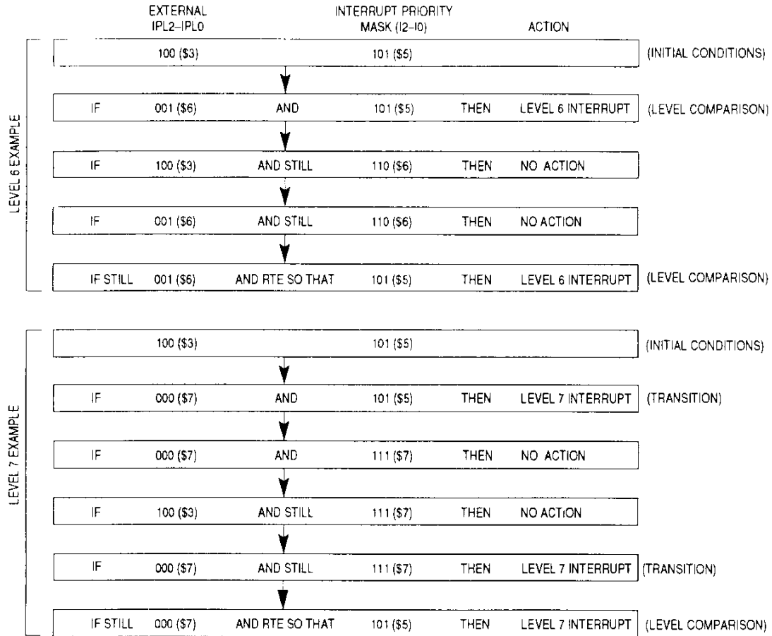
Figure 8-3. Interrupt Recognition Examples
