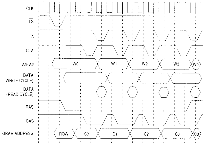
Figure 7-24. Using \overline{CLA} in a High-Speed DRAM Design
