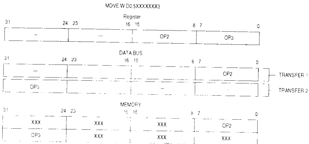
Figure 7-10. Example of Misaligned Word Transfer
