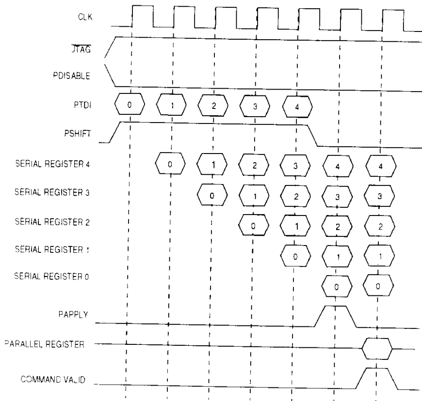
Figure 9-11. Interface Timing
