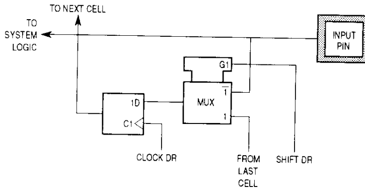
Figure 9-4. Observe-Only Input Pin Cell (I.Obs)
