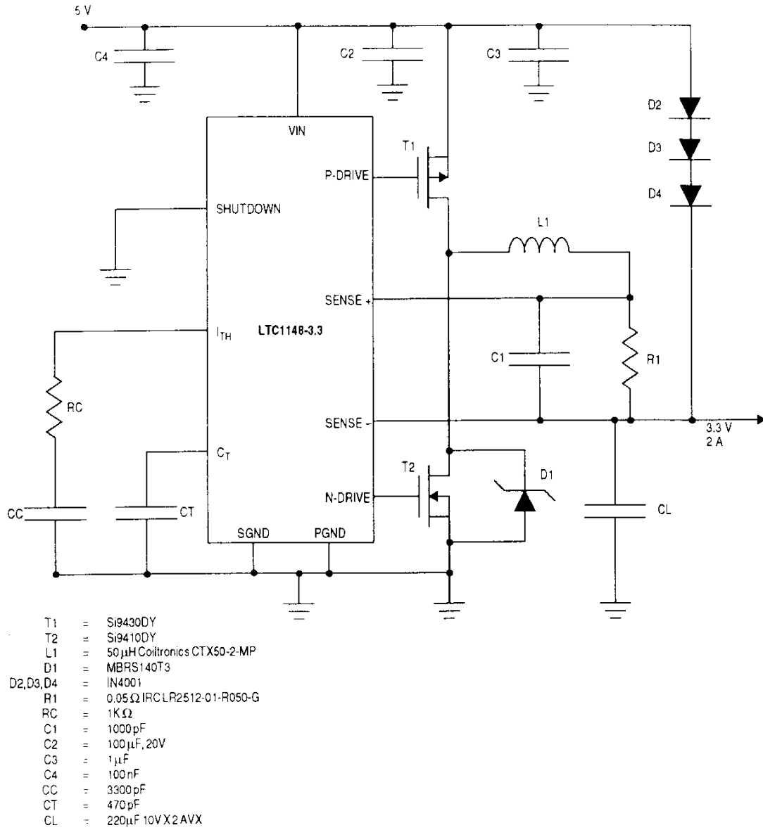
Figure 11-3. LTC1148 Voltage Regulator Solution
