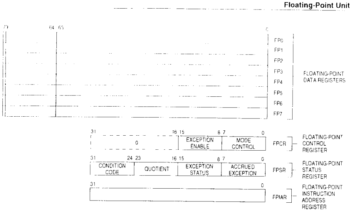
Figure 6-2. Floating-Point User Programming Model
