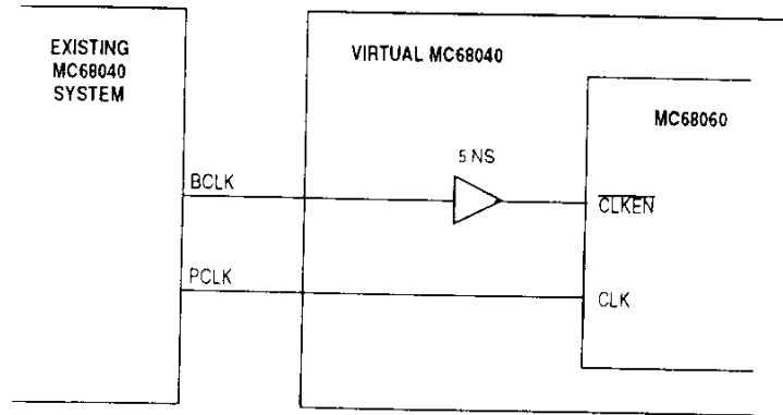
Figure 11-8. Simple CLK Generation
