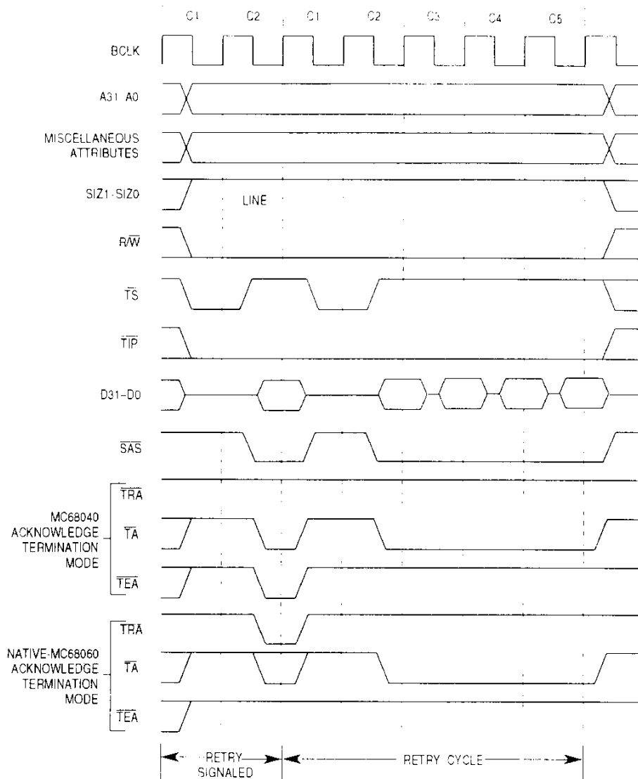
Figure 7-40. Line Write Retry Bus Cycle Timing
