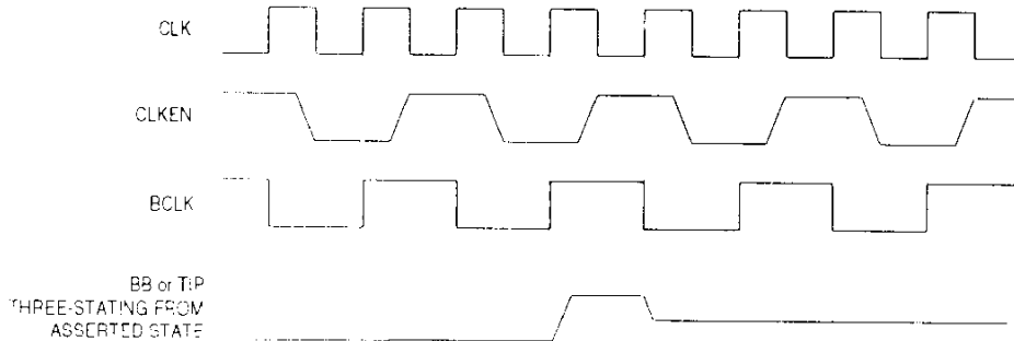
Figure 7-3. Half-Speed Clock
