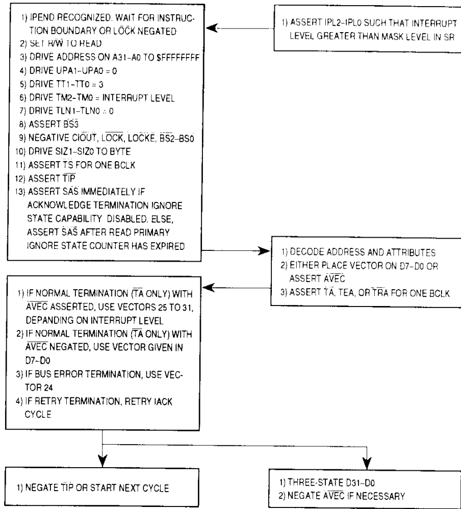
Figure 7-27. Interrupt Acknowledge Cycle Flowchart
