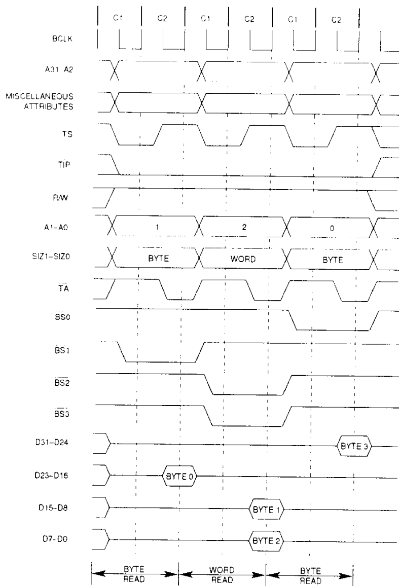
Figure 7-11. Misaligned Long-Word Read Bus Cycle Timing
