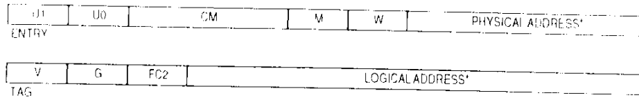
Figure 4-20. ATC Entry and Tag Fields
