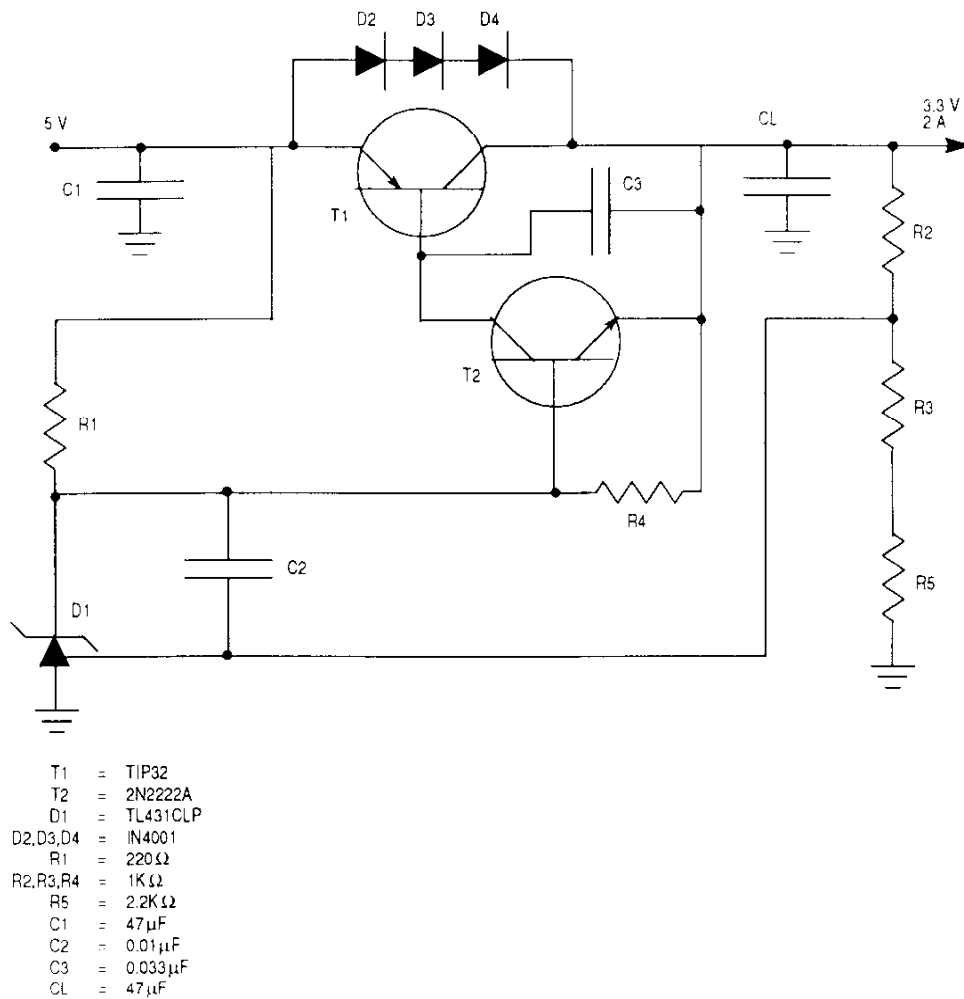
Figure 11-1. Linear Voltage Regulator Solution
