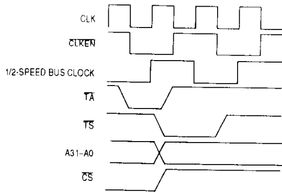
Figure 11-6. MC68060 Address Hold Time
