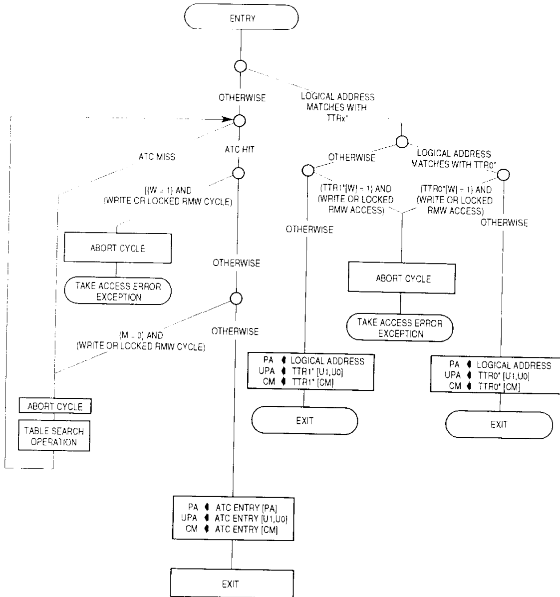
Figure 4-21. Address Translation Flowchart
