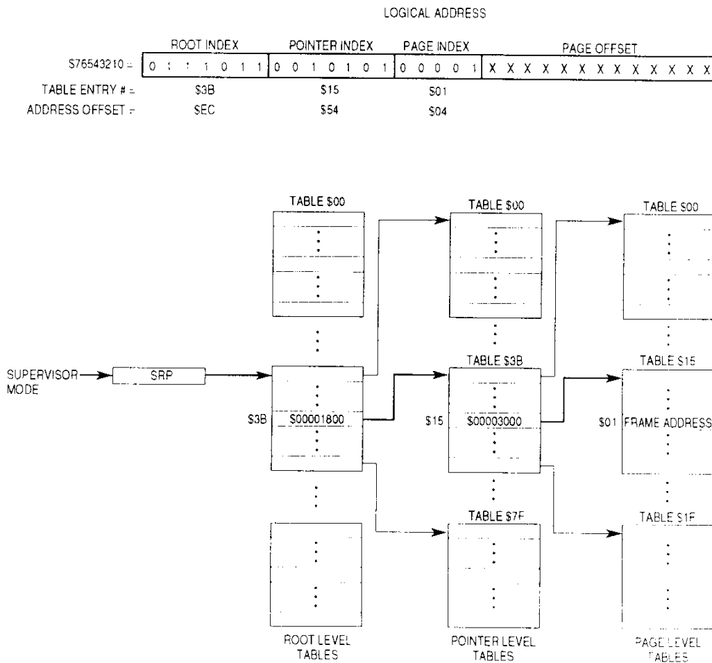
Figure 4-12. Example Translation Table
