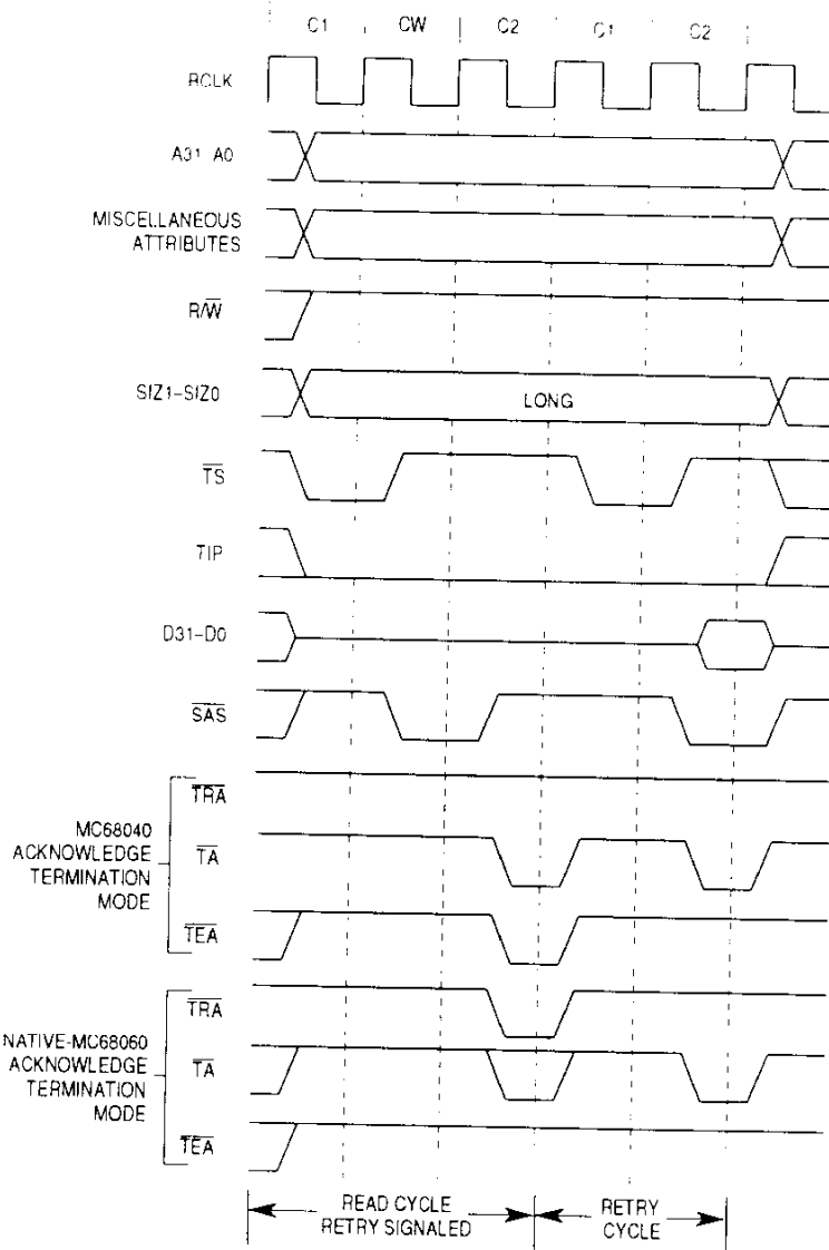
Figure 7-39. Retry Read Bus Cycle Timing
