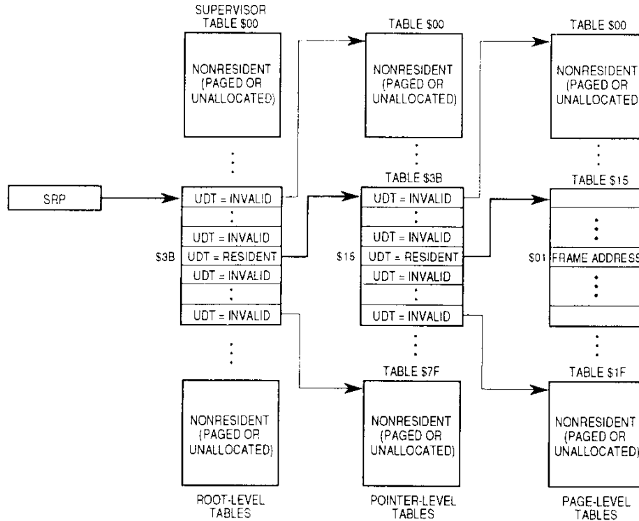
Figure 4-15. Translation Table with Nonresident Tables
