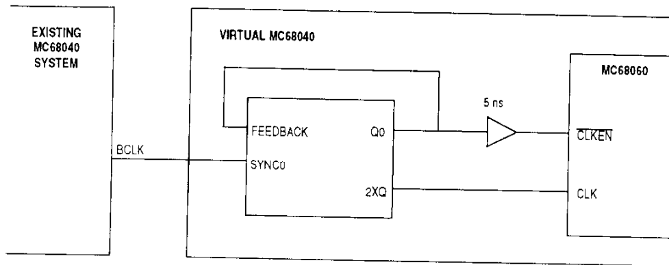
Figure 11-9. Generic CLK Generation
