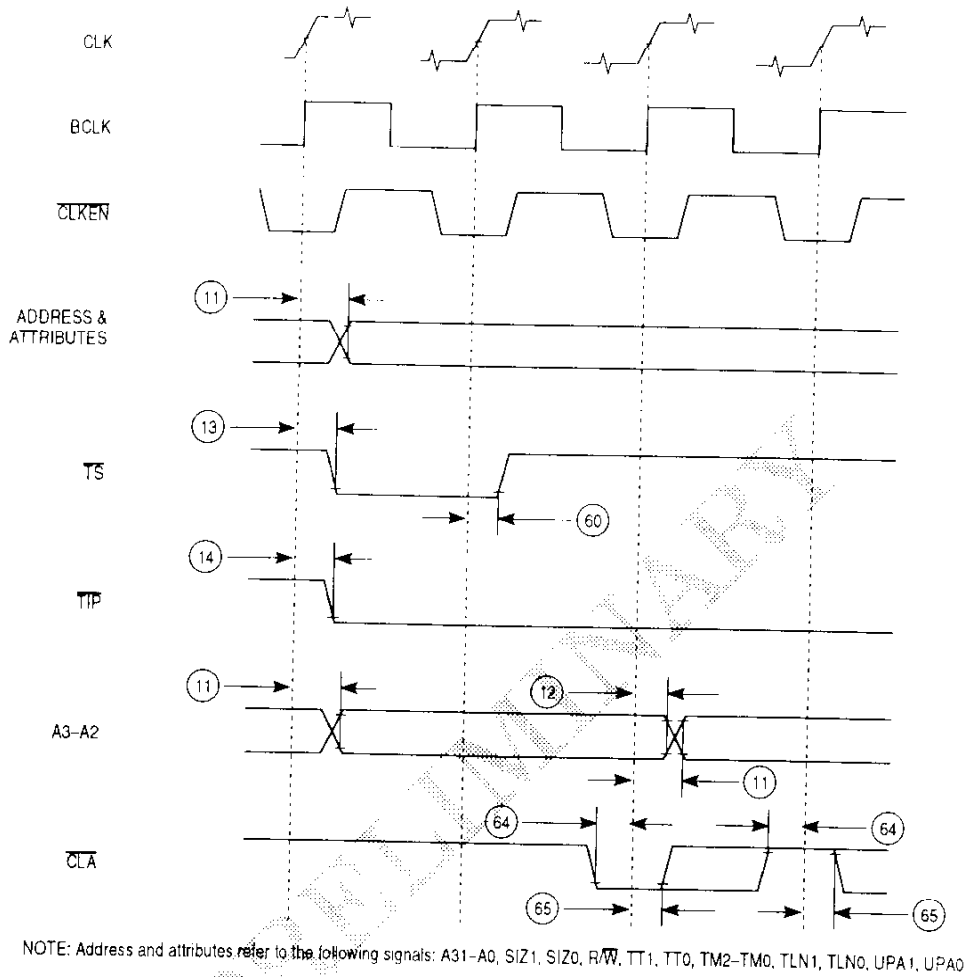
Figure 12-18. CLA Timing
