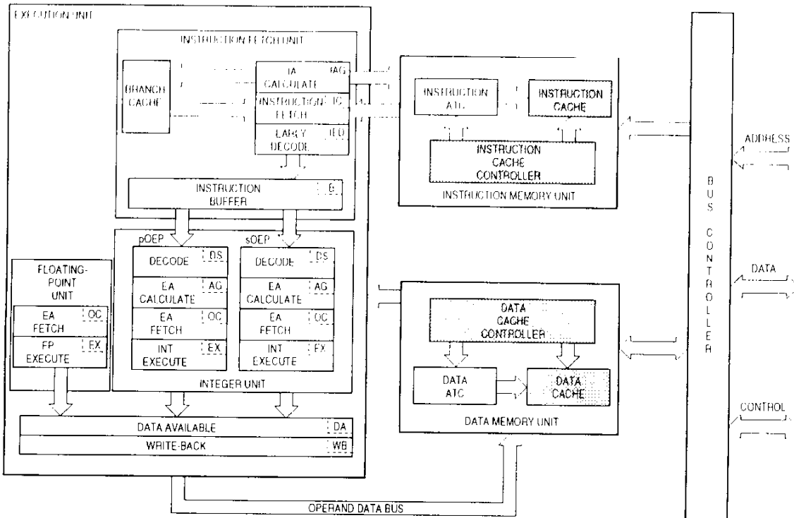
Figure 5-1. MC68060 Instruction and Data Caches
