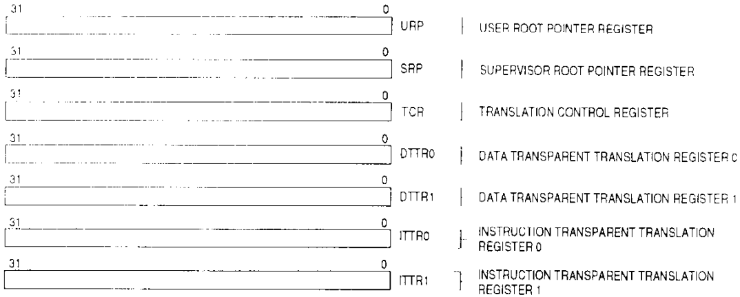
Figure 4-2. Memory Management Programming Model
