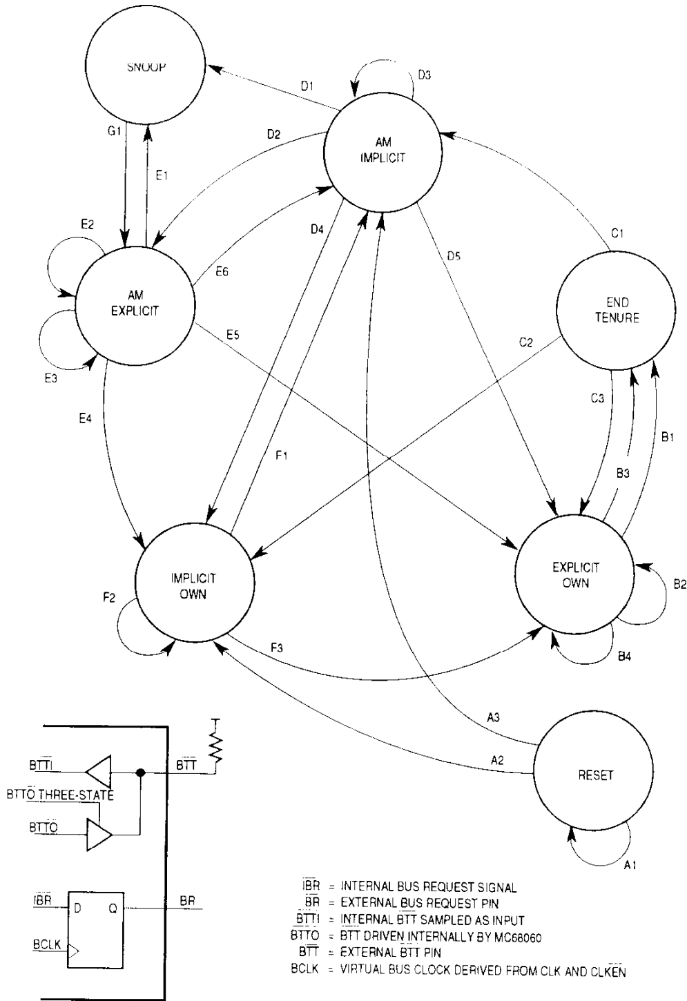
Figure 7-42. MC68060-Arbitration Protocol State Diagram
