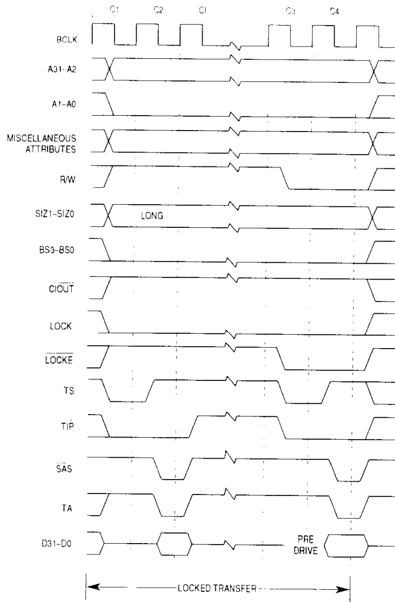
Figure 7-23. Locked Bus Cycle for TAS Instruction Timing
