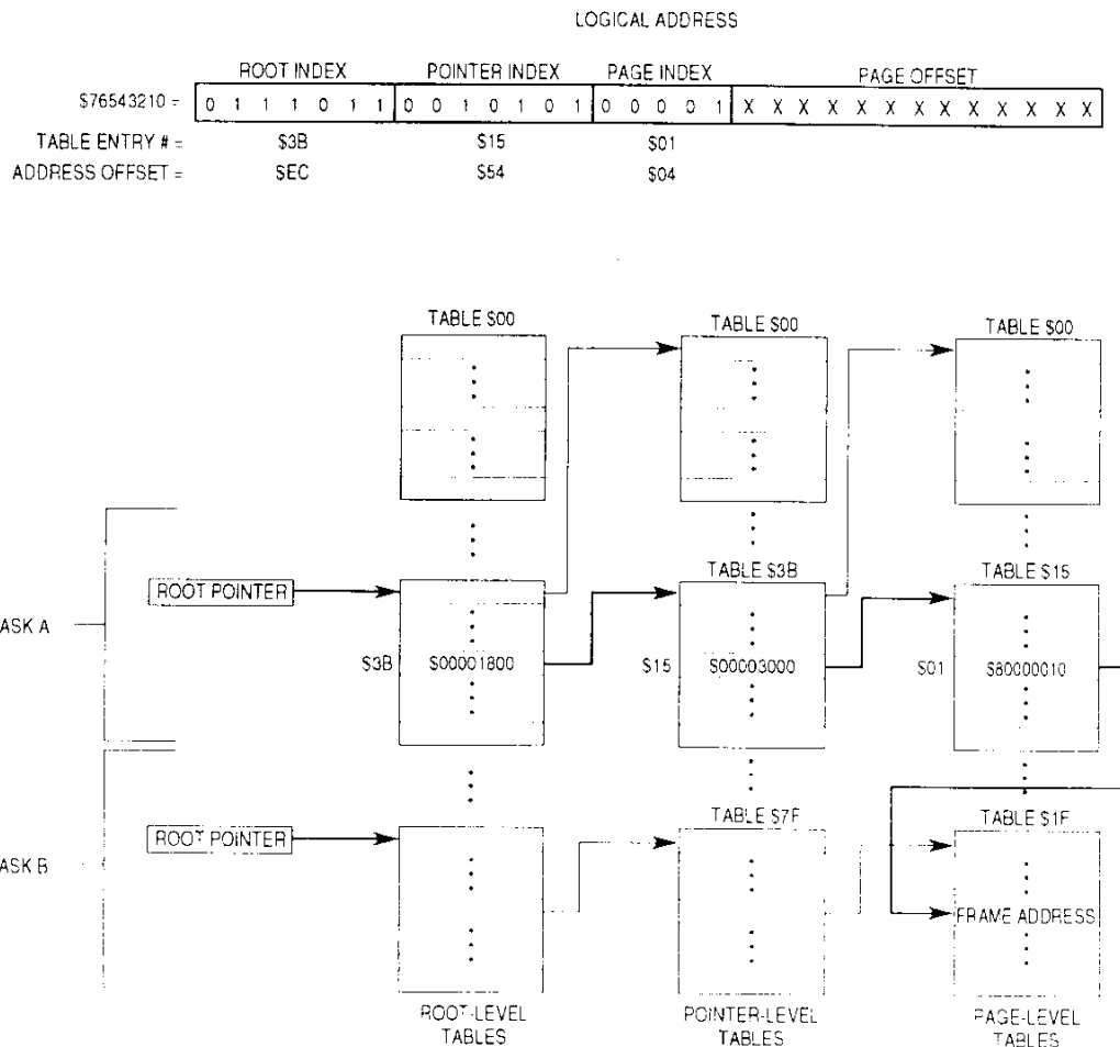
Figure 4-13. Translation Table Using Indirect Descriptors
