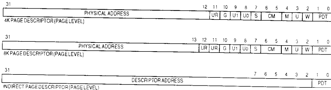
Figure 4-11. Page Descriptor Formats
