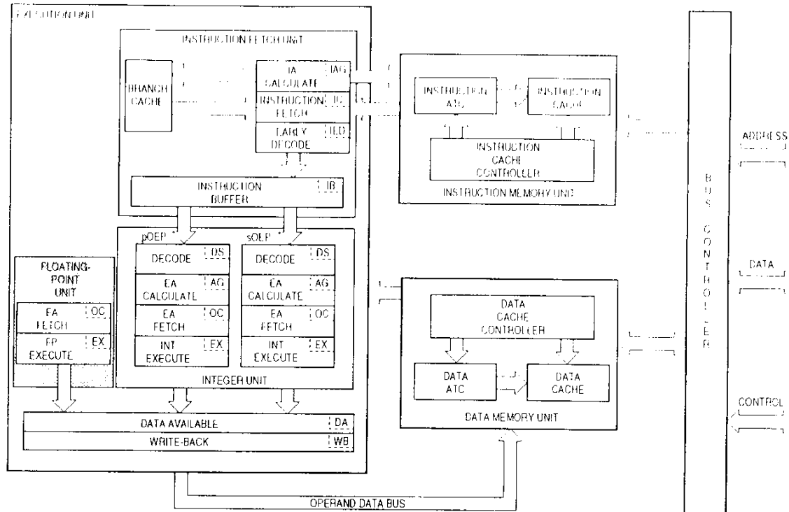
Figure 6-1. Floating-Point Unit Block Diagram
