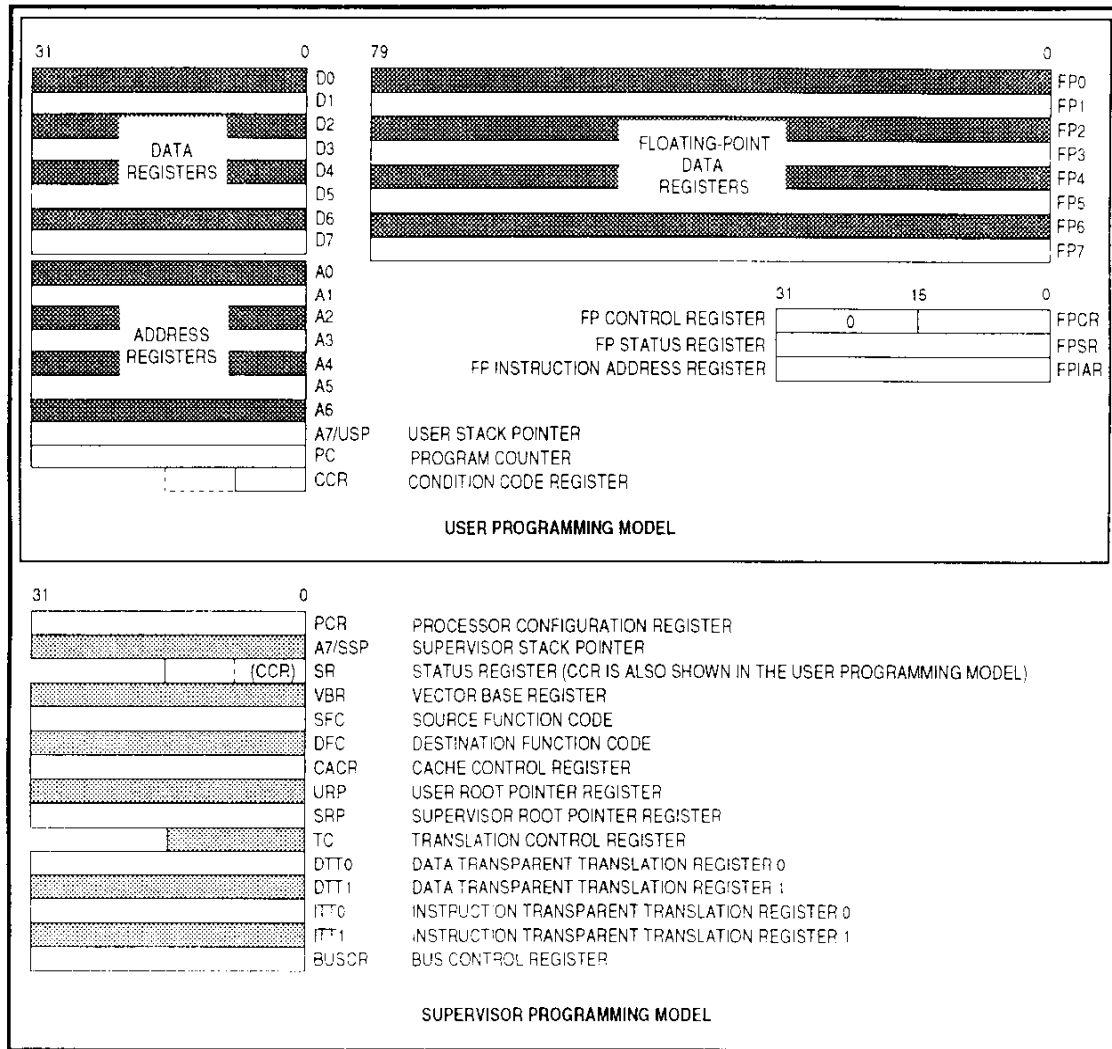
Figure 1-2. Programming Model
