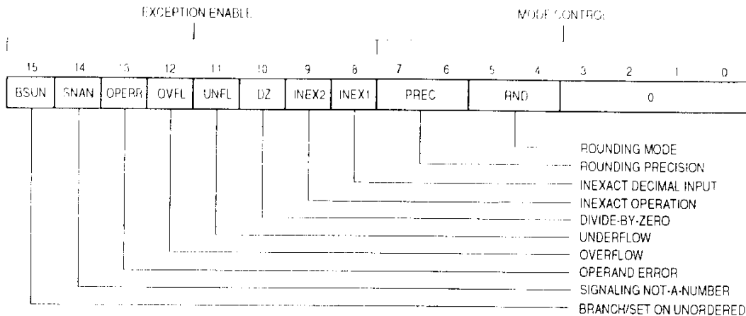
Figure 6-3. Floating-Point Control Register Format
