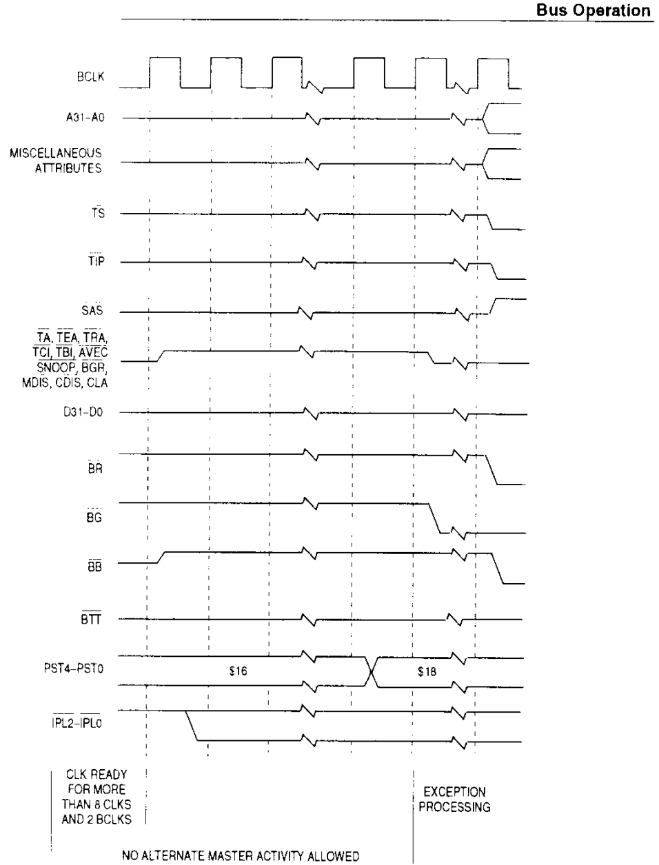
Figure 7-36. Exiting LPSTOP Mode Timing Diagram
