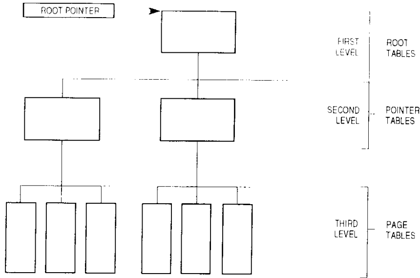
Figure 4-6. Translation Table Structure
