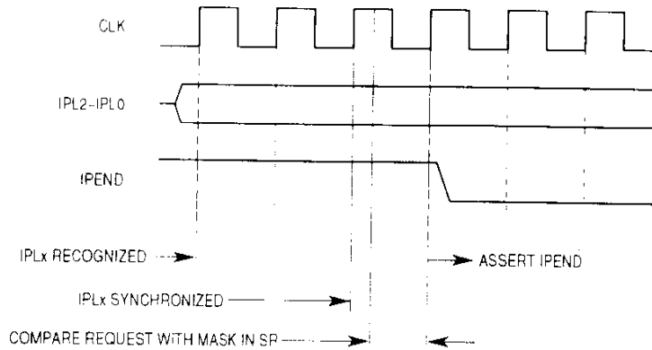
Figure 7-26. Assertion of \overline{IPEND}
