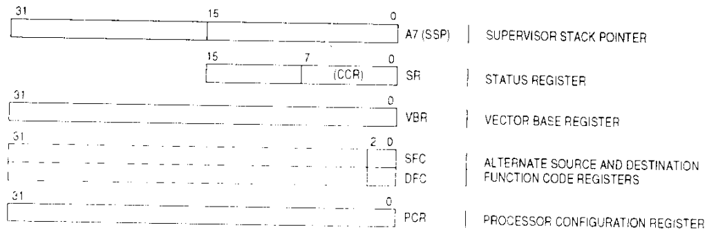
Figure 3-3. Integer Unit Supervisor Programming Model
