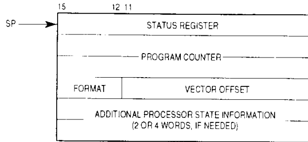
Figure 8-2. General Form of Exception Stack Frame
