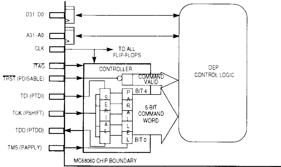
Figure 9-10. Debug Command Interface Schematic
