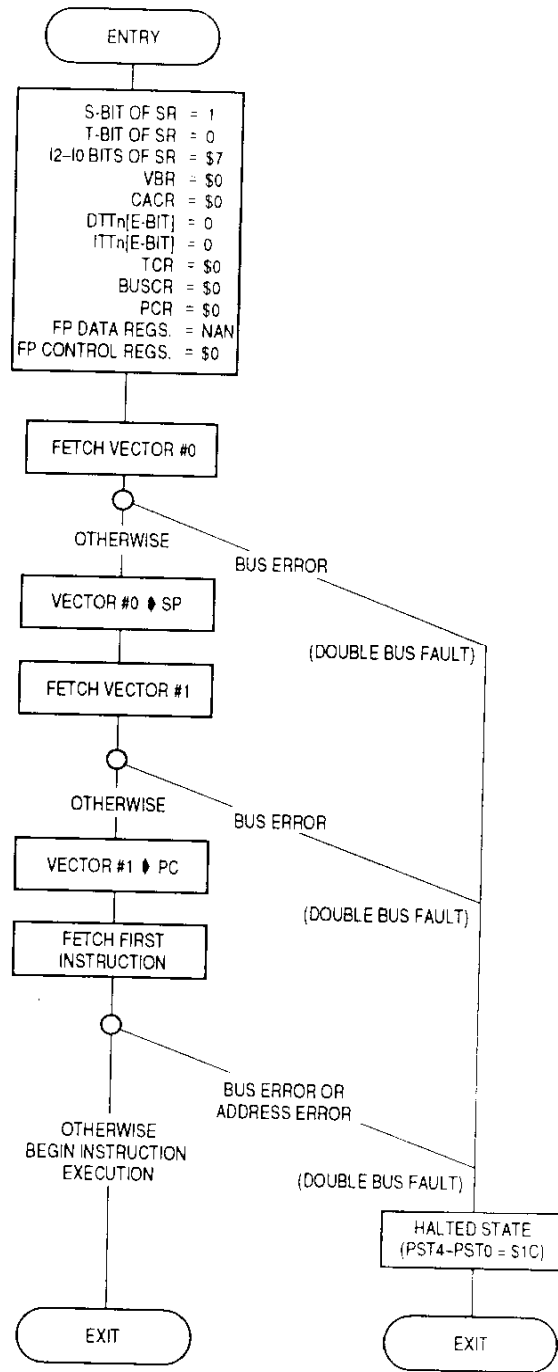
Figure 8-5. Reset Exception Processing Flowchart
