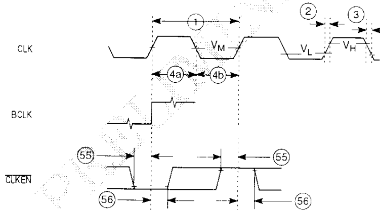
Figure 12-12. Clock Input Timing Diagram
