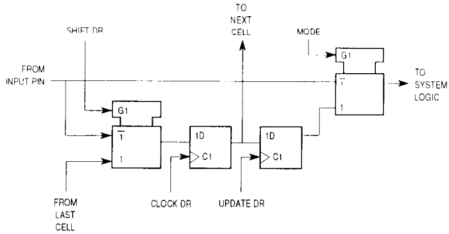
Figure 9-5. Input Pin Cell (I.Pin)
