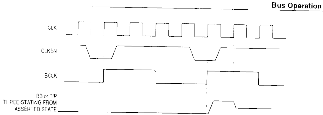
Figure 7-4. Quarter-Speed Clock
