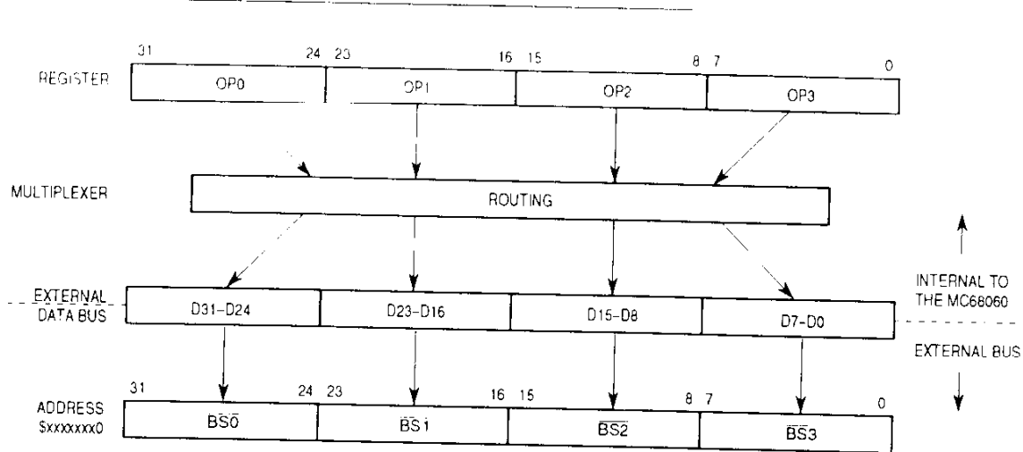
Figure 7-7. Data Multiplexing
