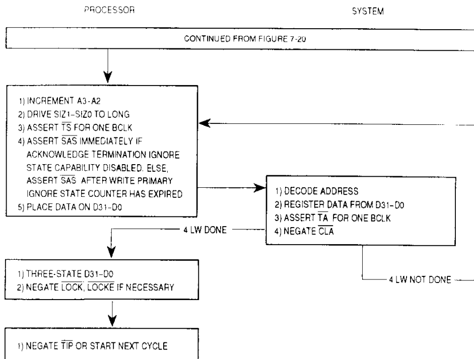
Figure 7-21. Line Write Burst-Inhibited Cycle Flowchart
