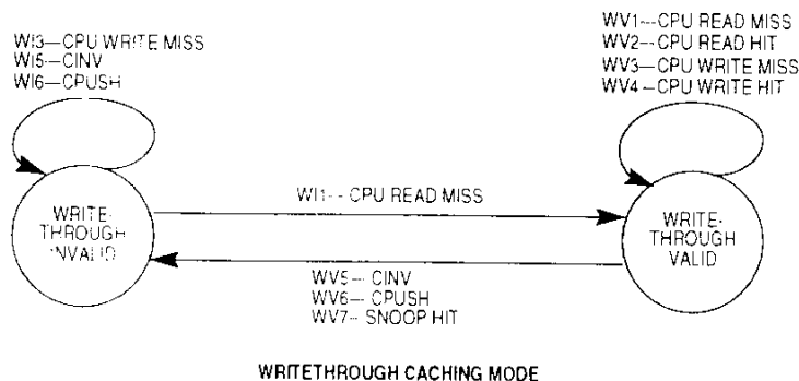
Figure 5-7. Data Cache Line State Diagrams
