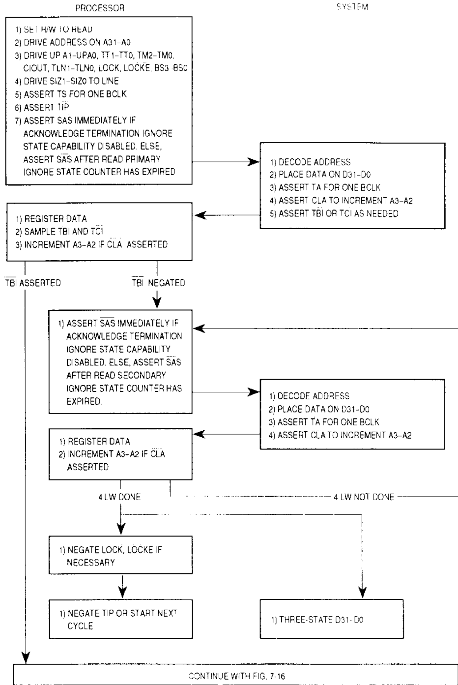
Figure 7-14. Line Read Cycle Flowchart
