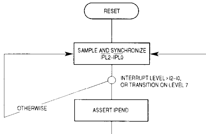
Figure 7-25. Interrupt Pending Procedure
