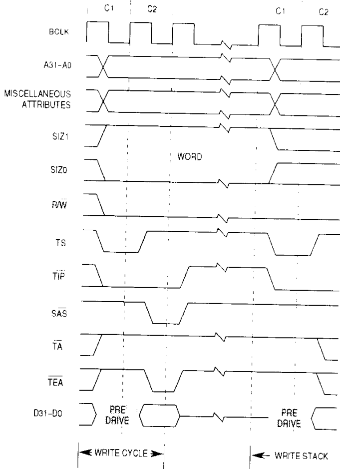
Figure 7-37. Word Write Access Bus Cycle Terminated with \overline{TEA} Timing
