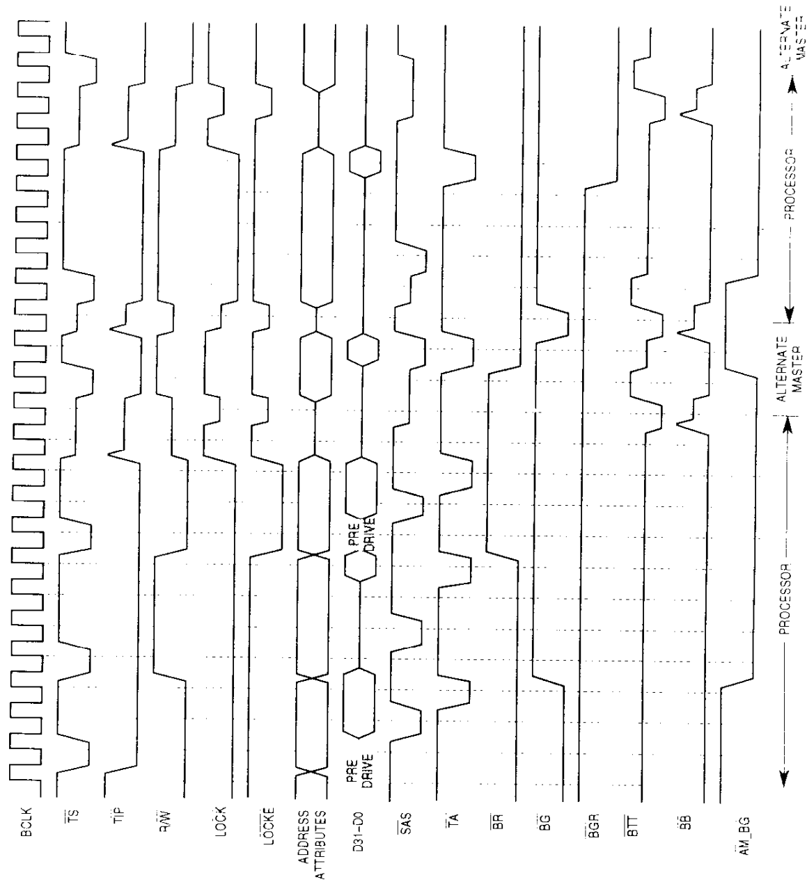
Figure 7-46. Effect of \overline{BGR} on Locked Sequences
