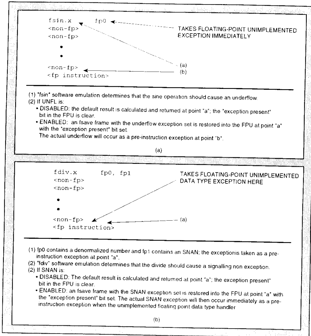
Figure C-9. Disabled vs. Enabled Exception Actions
