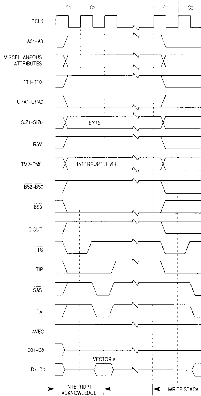
Figure 7-28. Interrupt Acknowledge Bus Cycle Timing
