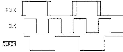
Figure 11-10. MC68040 BCLK to \overline{\text{CLKEN}} Relationship
