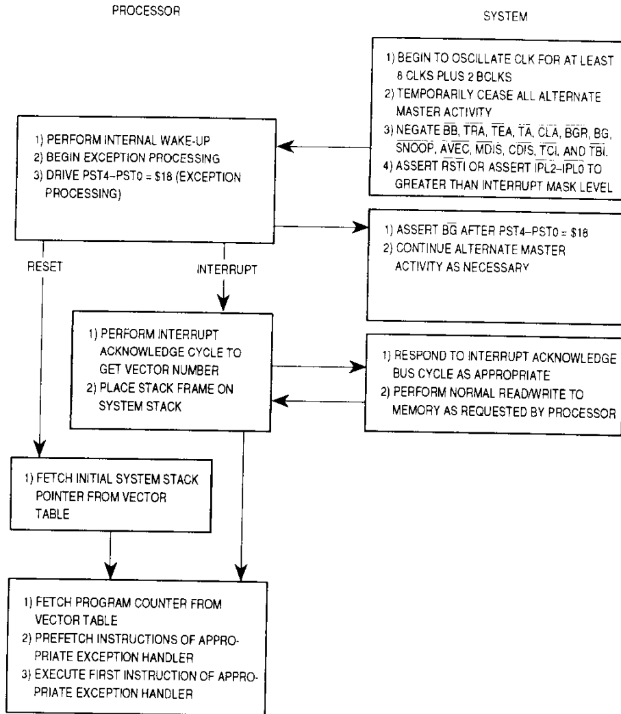
Figure 7-35. Exiting LPSTOP Mode Flowchart
