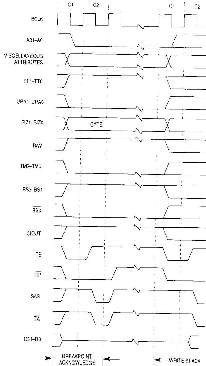
Figure 7-31. Breakpoint Interrupt Acknowledge Bus Cycle Timing
