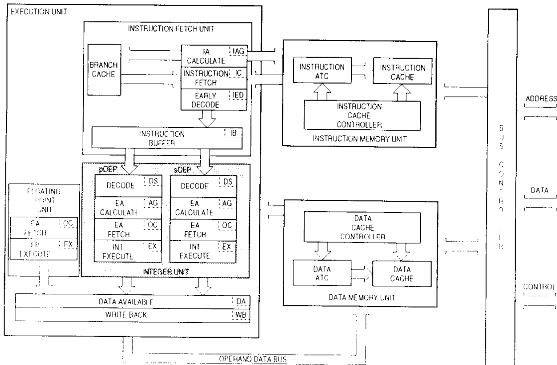
Figure 3-1. MC68060 Integer Unit Pipeline
