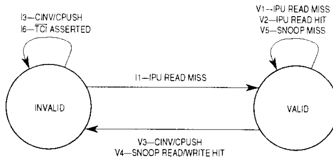
Figure 5-6. Instruction Cache Line State Diagram
