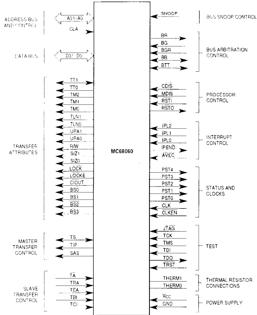
Figure 2-1. Functional Signal Groups
