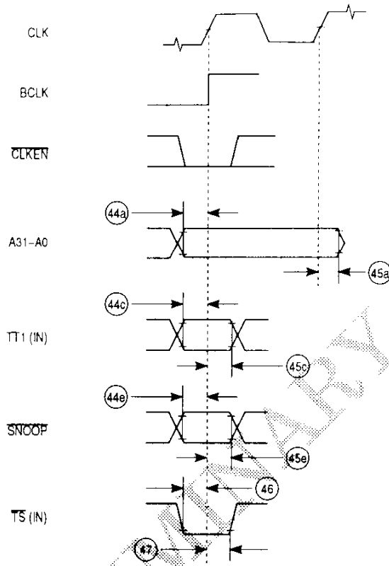
Figure 12-19: Snoop Timing
