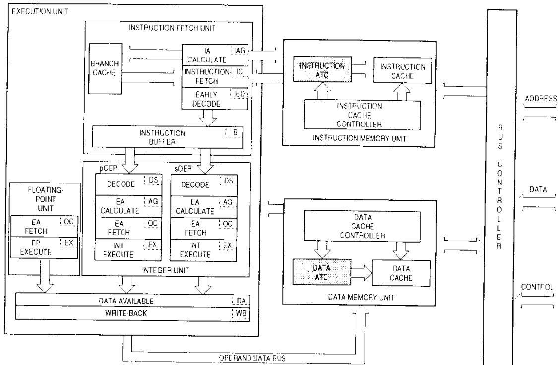
Figure 4-1. Memory Management Unit
