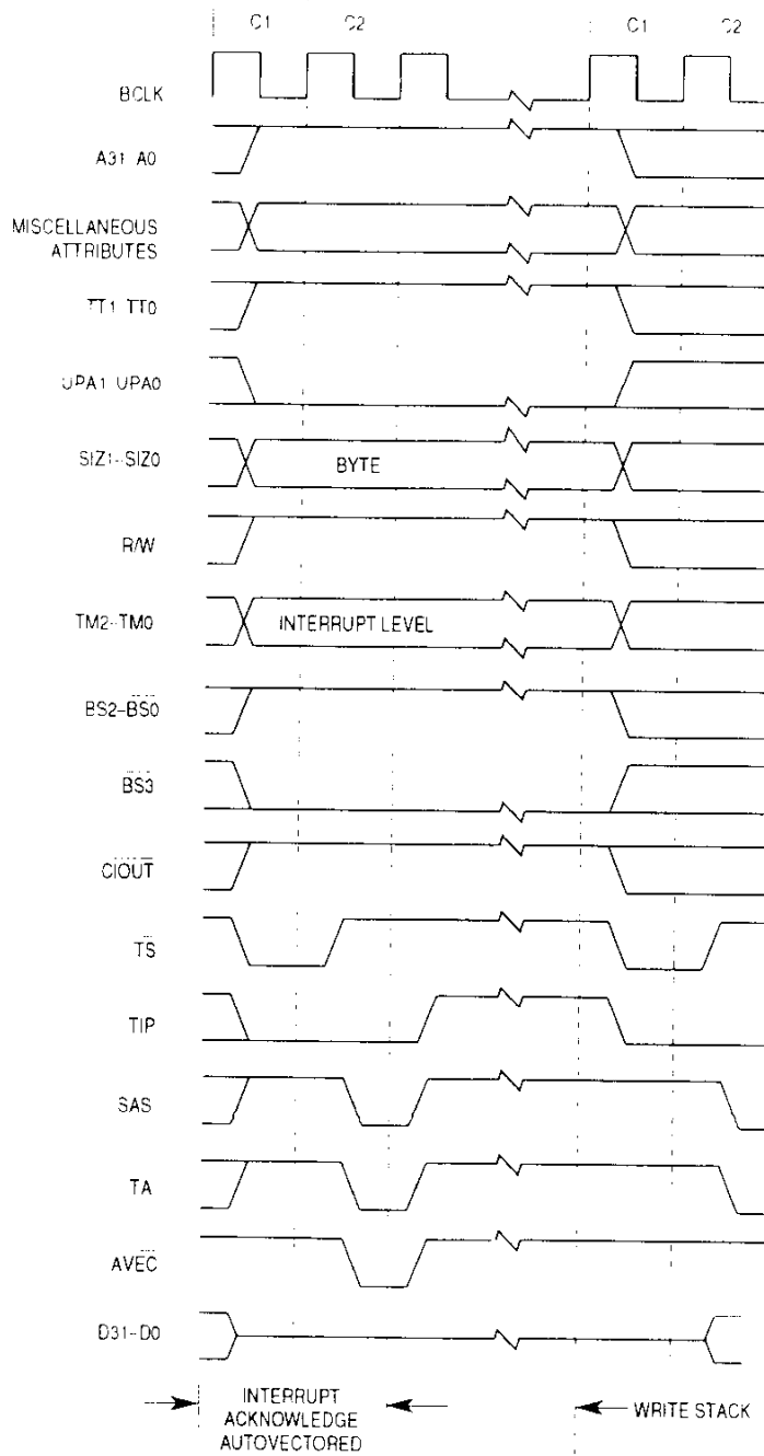
Figure 7-29. Autovector Interrupt Acknowledge Bus Cycle Timing
