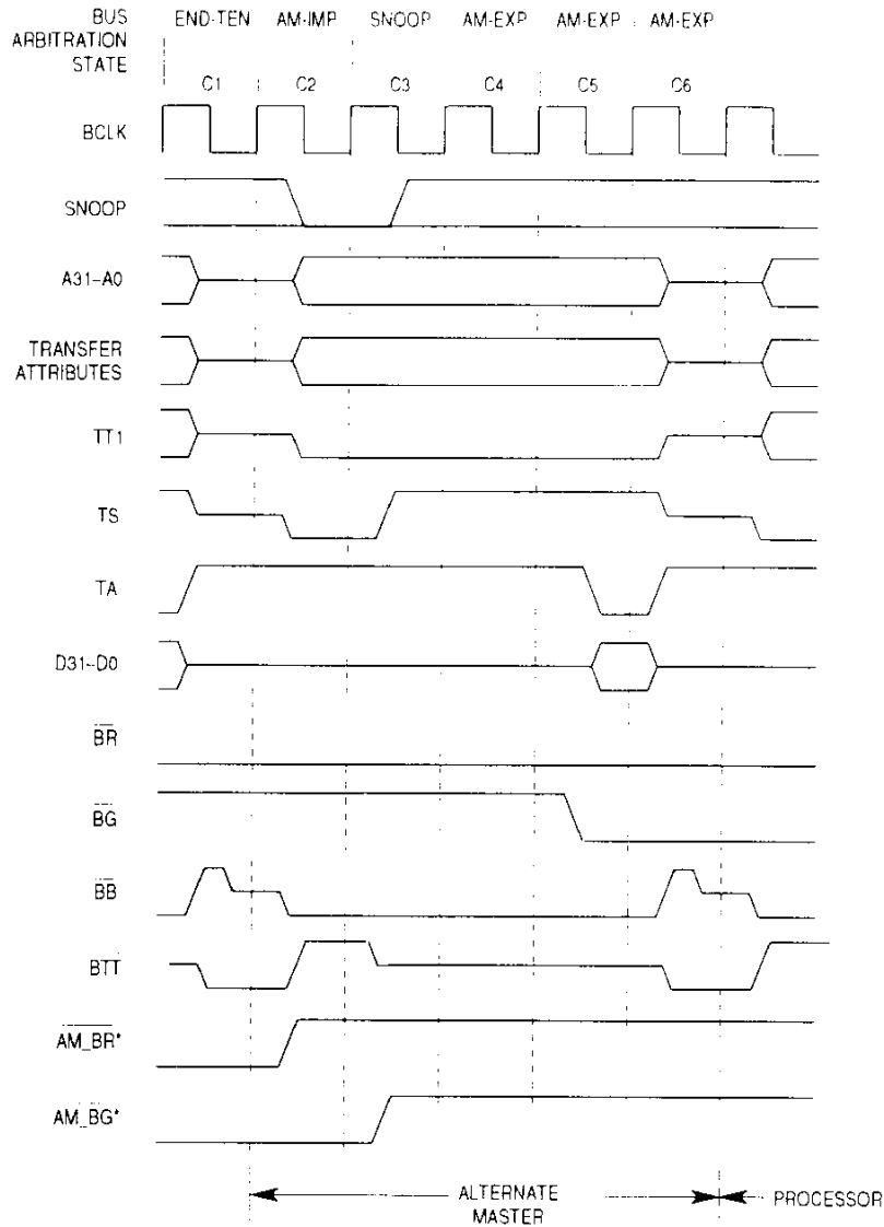
Figure 7-47. Snooped Bus Cycle
