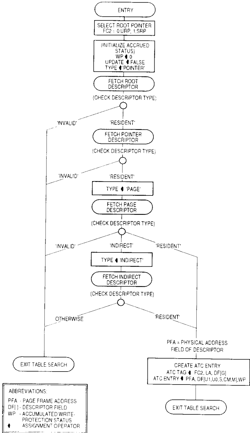
Figure 4-8. Detailed Flowchart of Table Search Operation
