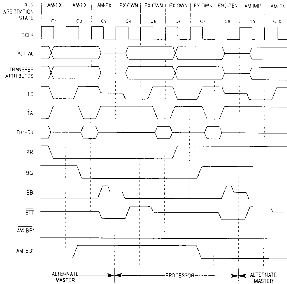
Figure 7-43. Processor Bus Request Timing
