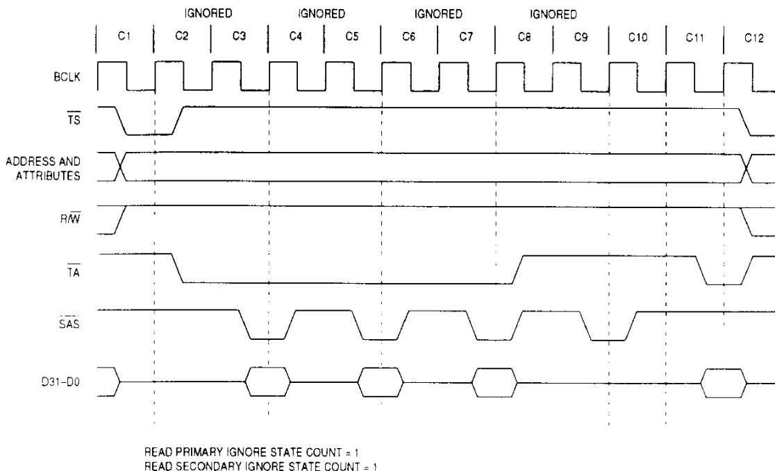
Figure 7-51. Acknowledge Termination Ignore State Example
