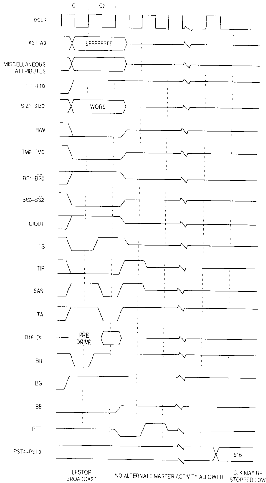
Figure 7-33. LPSTOP Broadcast Bus Cycle Timing, \overline{BG} Negated
