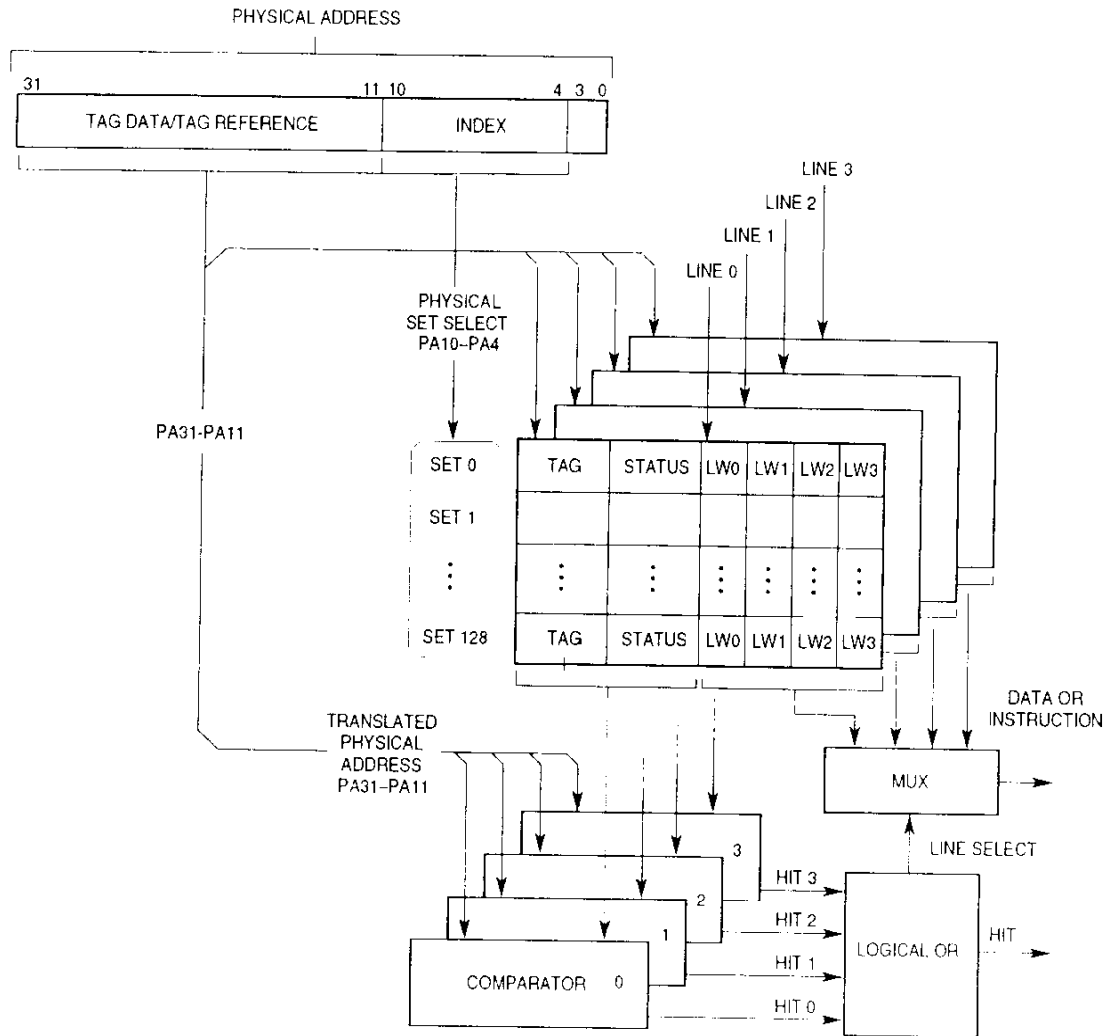
Figure 5-4. Caching Operation
