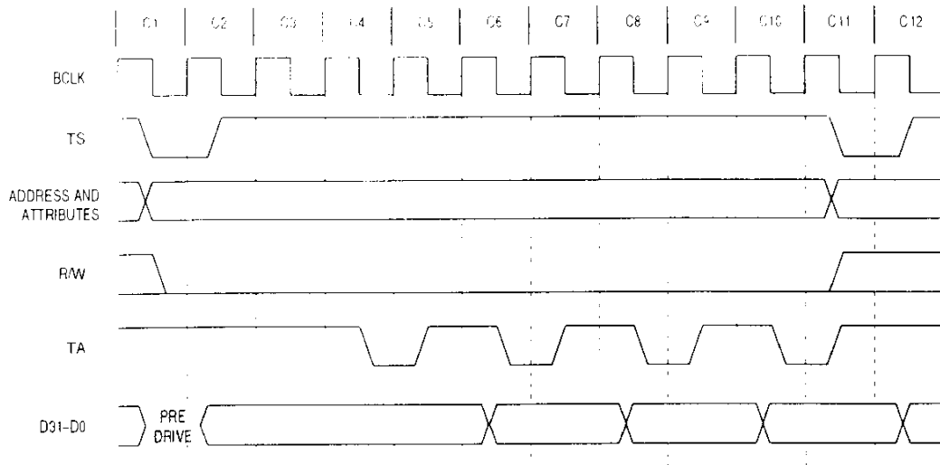
Figure 7-52. Extra Data Write Hold Example
