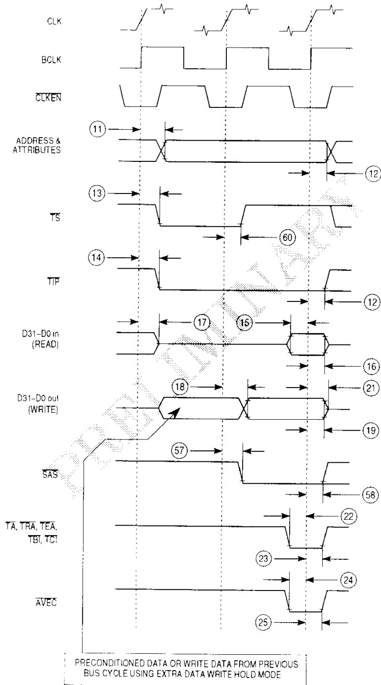
Figure 12-15. Read/Write Timing
