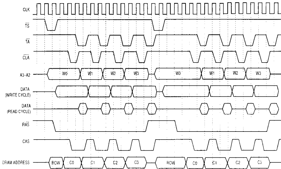
Figure 11-11. DRAM Timing Analysis
