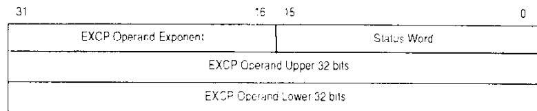
Figure 6-10. Floating-Point State Frame
