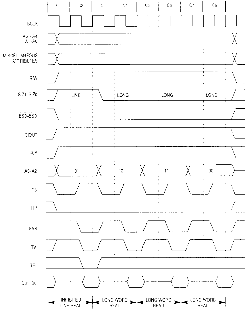
Figure 7-17. Burst-Inhibited Line Read Bus Cycle Timing
