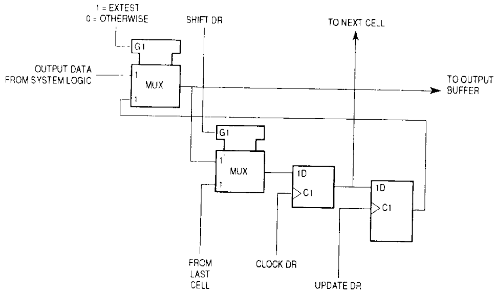
Figure 9-3. Output Pin Cell (O.Pin)
