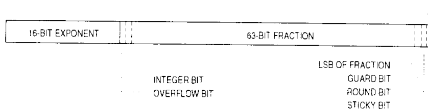
Figure 6-8. Intermediate Result Format
