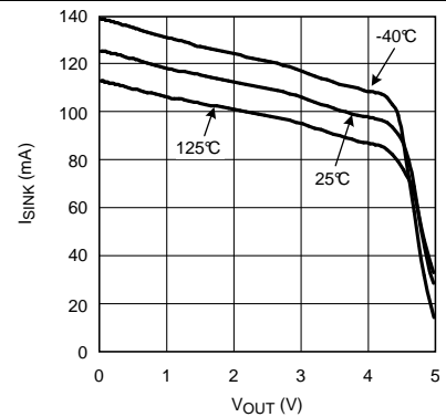
Figure 26. Sinking Current vs. V_{OUT} (LMH6626)
