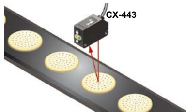
Detecting a biscuit
