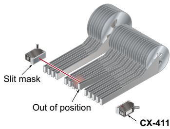
Detecting out of position tape feeder cassette
