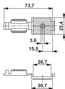
Dimensioned drawing
