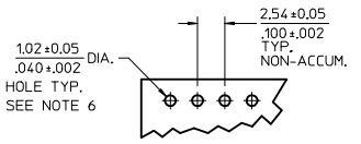
TYP. HOLE PATTERN FOR 1.57/0.062 THK. PCB
