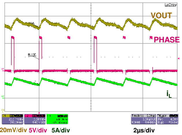
Figure 11: CCM (IOUT = 6A)
