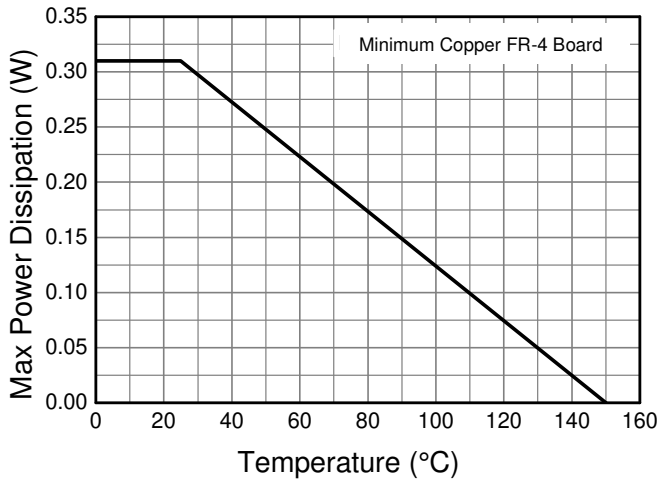
Derating Curve
