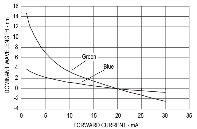
Figure 4. Relative Dominant Wavelength vs. DC Forward Current
