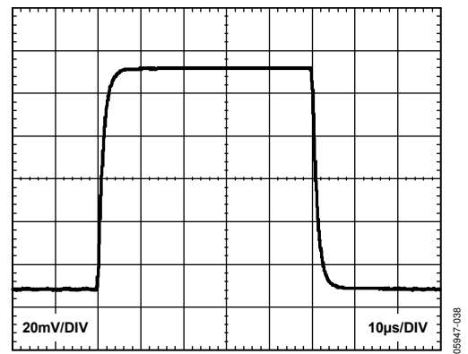
Figure 38. Small Signal Response, G = 100 , R_L = 2\text{ k}\Omega , C_L = 100\text{ pF}
