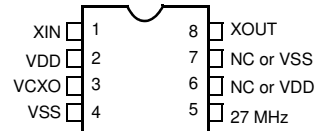
Figure 1. CY2410-1, CY2410-5 8-pin SOIC
