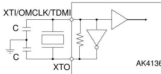
Note: Refer to Table 5 for the capacitor and resistance values for the X'tal oscillator. Figure 26. X'tal (XTI) Mode
