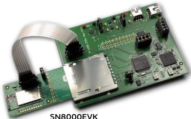
SN8000EVK (P/N 88-00153-85 & 88-00153-87)
