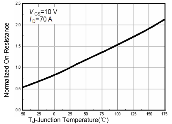
Figure 4. Rdson-Junction Temperature
