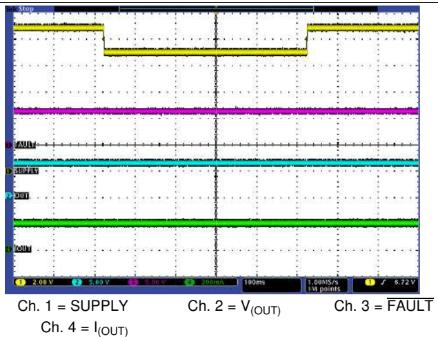
Figure 10. Transient Undervoltage
