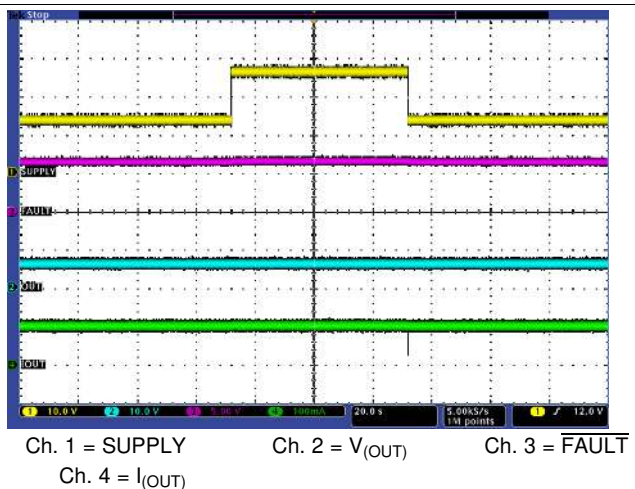
Figure 12. Jump Start
