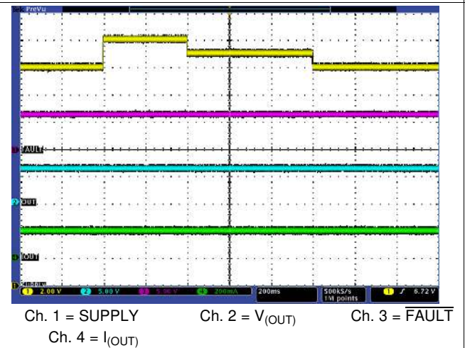
Figure 11. Transient Overvoltage
