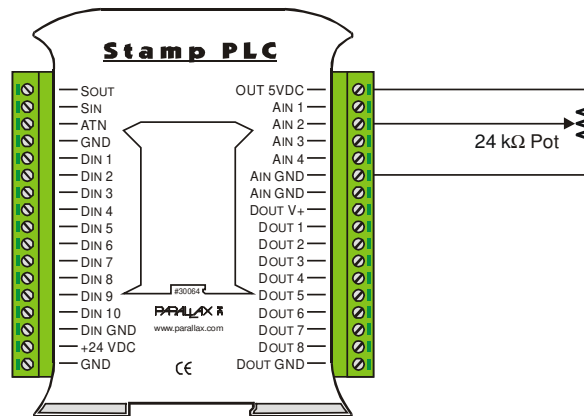
Figure 9: Stamp PLC to Potentiometer
