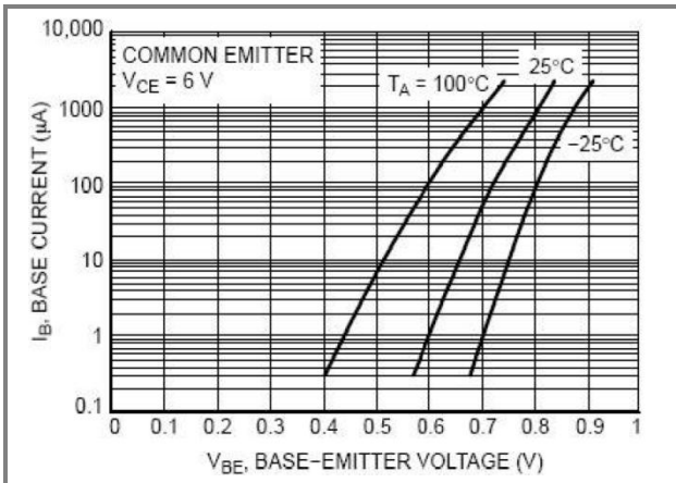
Fig.10 Base-Emitter Voltage
