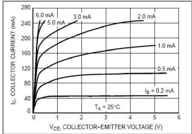
Fig.7 Collector Current
