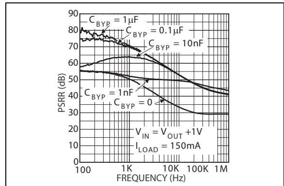
FIGURE 2-30: Power Supply Rejection Ratio vs. C_{BYPASS} .
