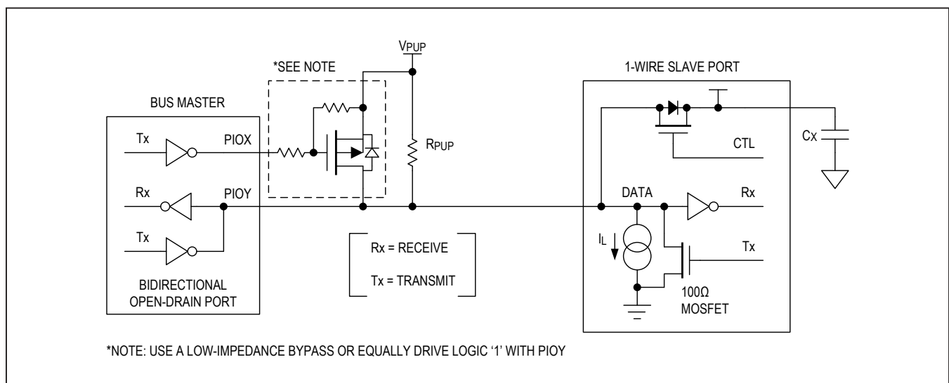
Figure 4. Hardware Configuration
