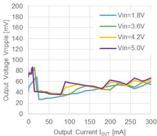
RP517x121x, Ta=25°C
