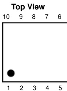
RP517K [DFN(PL)2527-10] Pin Configuration
