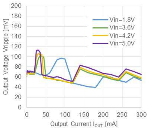
RP517x031x, Ta=25°C
