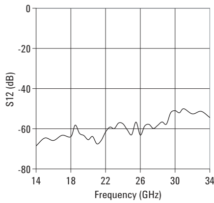
Figure 2. Typical Isolation
