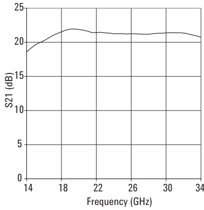
Figure 1. Typical Gain
