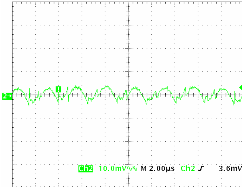
Figure 11. Ripple
