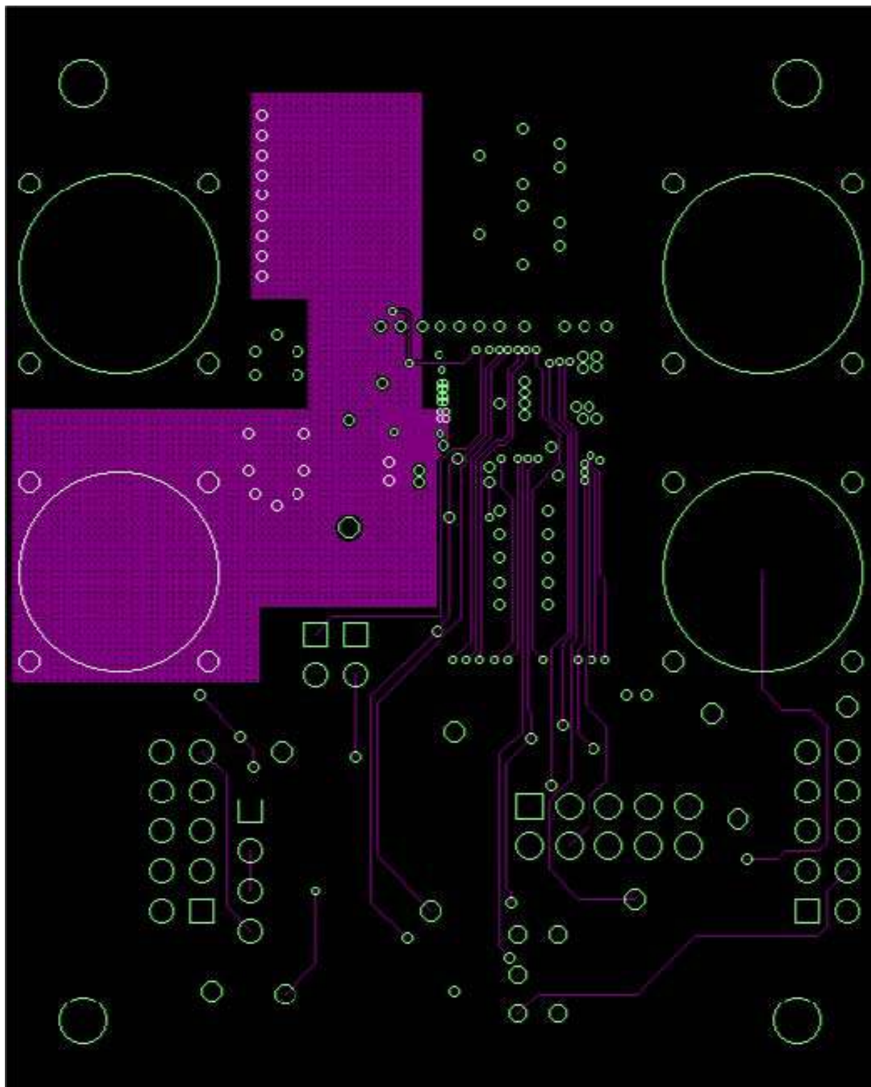
Figure 8. PCB – Inner Layer 2 (Viewed from Top)
