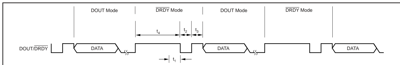
FIGURE 12. \overline{DOUT/DRDY} Partitioning.
