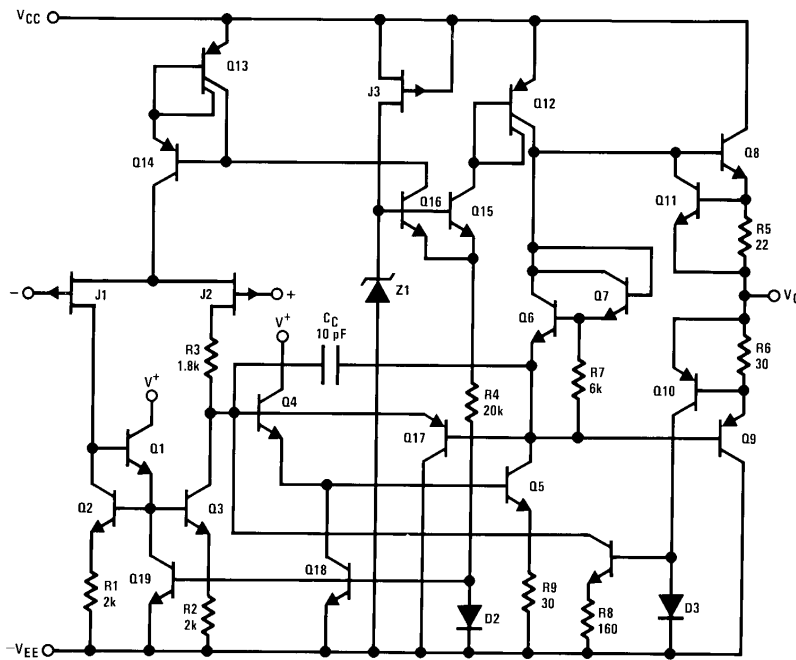
Figure 28. 1/2 Dual LF412-N-MIL
