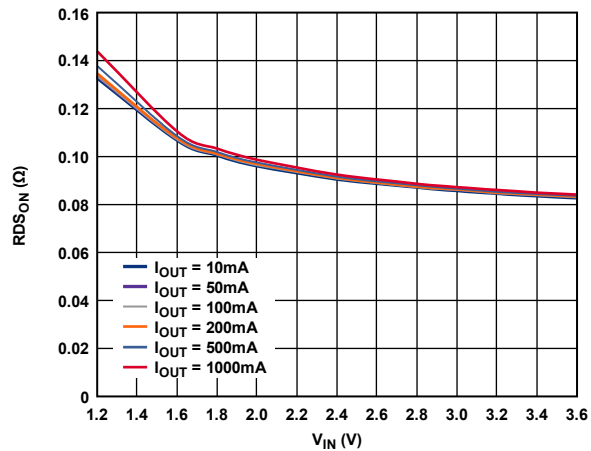
Figure 6. 6-Lead LFCSP R DS(ON) vs. Input Voltage, V IN
