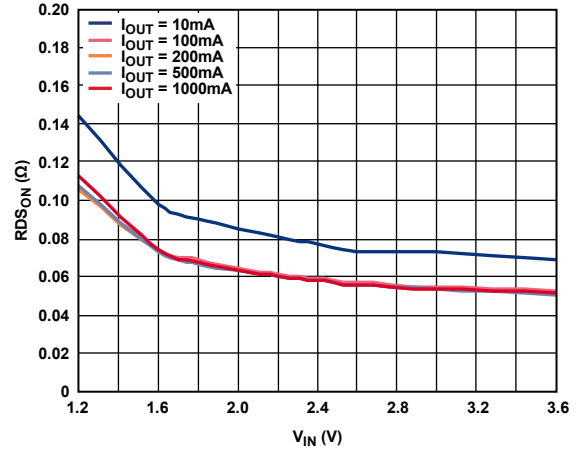
Figure 5. 4-Ball WLCSP R DS(ON) vs. Input Voltage, V IN
