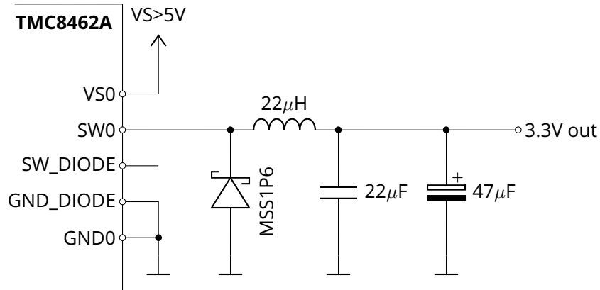
Figure 22: External circuit for switching regulator 0 with VS0 > 5V
