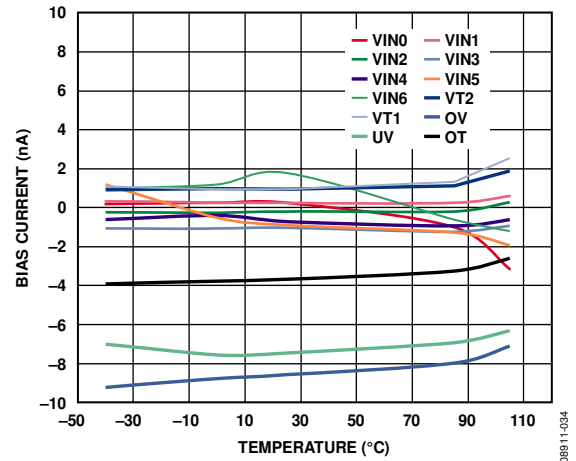
Figure 31. Input Bias Current vs. Temperature
