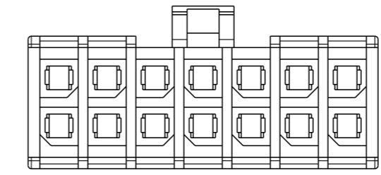
6POS8P(14P)
