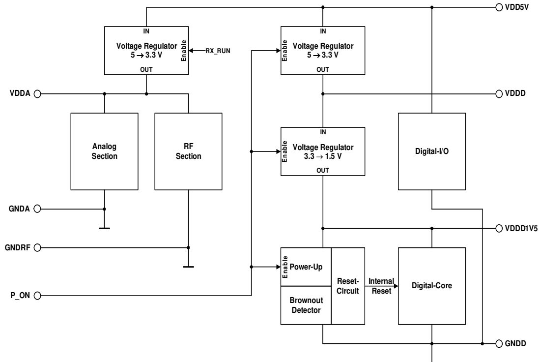
Figure 40 Power Supply
