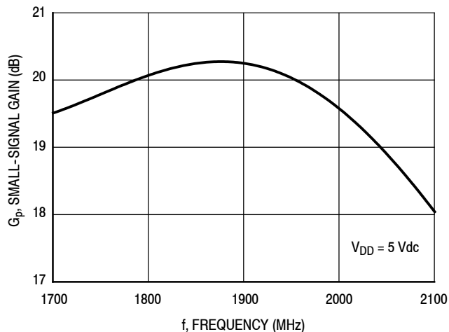
Figure 21. Small-Signal Gain (S21) versus Frequency
