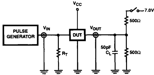
FIGURE 5. TEST CIRCUIT
