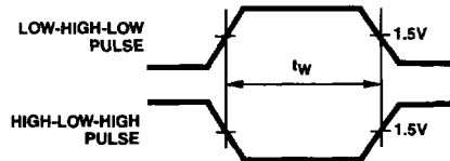
FIGURE 7. PULSE WIDTH
