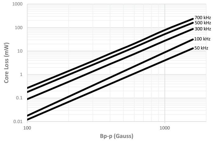
HCM1A0503V2-R68-R
