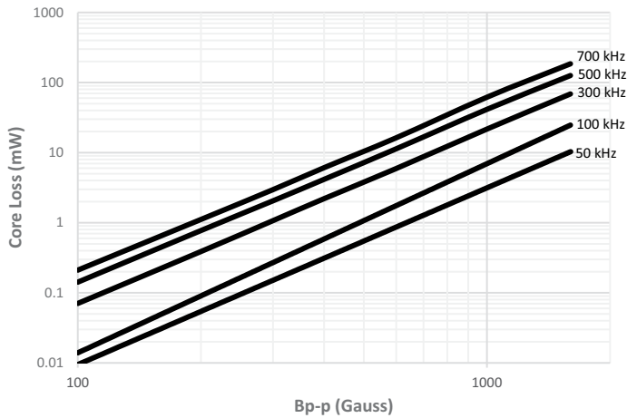
HCM1A0503V2-R75-R
