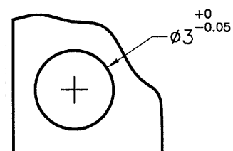
MOUNTING HOLE
