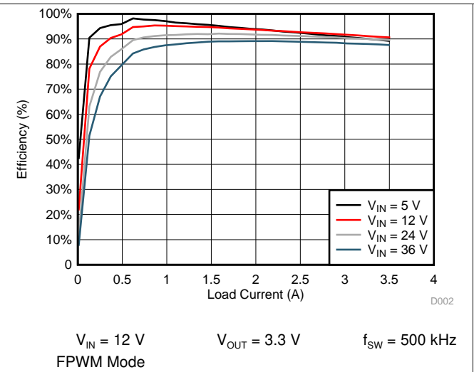
Figure 10. LM76003 Efficiency
