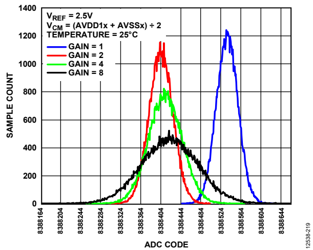
Figure 19. Noise Histogram at 4 kSPS, Low Power Mode
