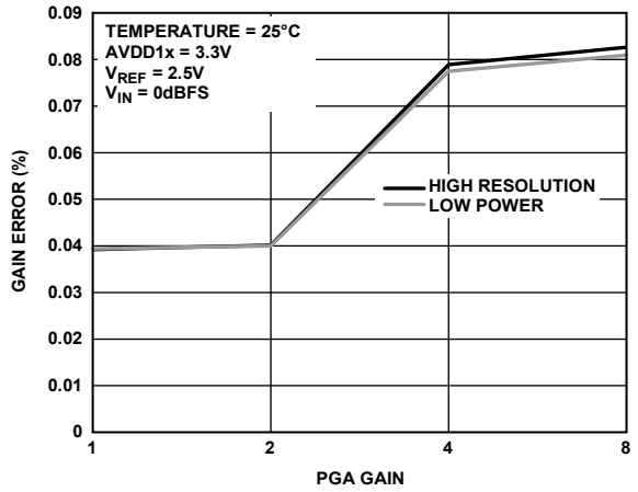
Figure 51. Channel Gain Mismatch, High Resolution Mode
