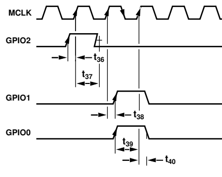
Figure 6. GPIOs for SRC Update Timing Diagram
