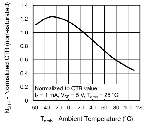
Fig. 10 - Normalized Current Transfer Ratio vs. Ambient Temperature (non-saturated)
