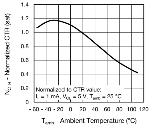
Fig. 9 - Normalized Current Transfer Ratio vs. Ambient Temperature (saturated)
