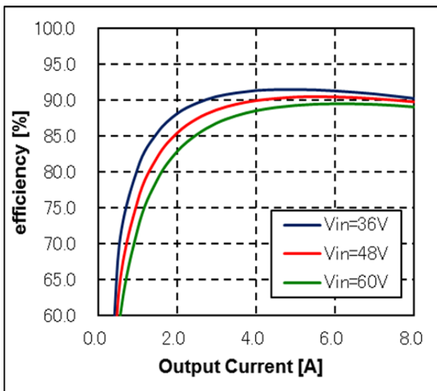
Fig-2: Efficiency vs. load current and input voltage for power module mounted horizontally with airflow from pin 1 to pin 3 at a rate of 400LFM (2.0m/s) and T_a=25^{\circ}C .
