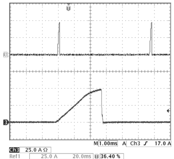
Fig-12: Load current (top trace, 25A/div, 20ms/div) into a 10m \Omega short circuit during restart, at V_{in} = 48V . Bottom trace (25A/div, 1ms/div) is an expansion of the top trace.
