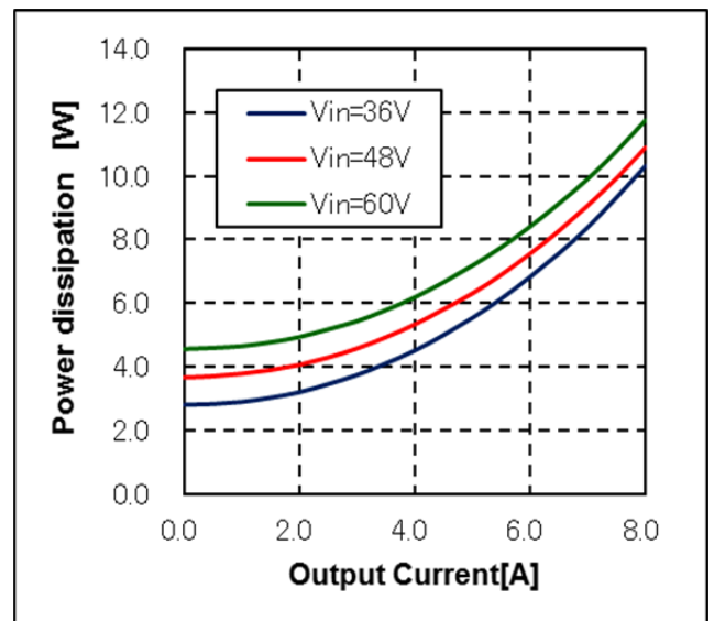
Fig-3: Power dissipation vs. load current and input voltage for power module mounted horizontally with airflow from pin 1 to pin 3 at a rate of 400LFM (2.0m/s) and T_a=25^{\circ}C .
