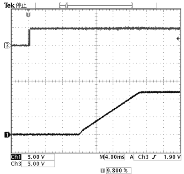
Fig-5: Turn-on transient at full rated load current (resistive) plus 4700uF at Vin=48V, triggered via ON/OFF pin. Top trace: ON/OFF signal (5V/div). Bottom trace: output voltage (5V/div). Time scale: 4ms/div
