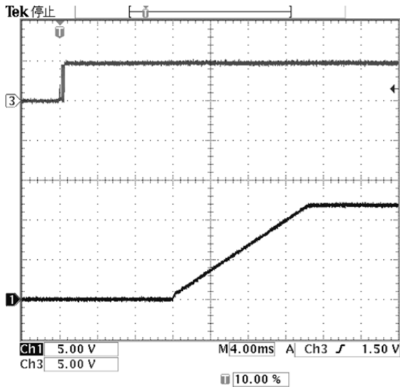
Fig-4: Turn-on transient at full rated load current (resistive) with 47uF ceramic capacitor at Vin=48V, triggered via ON/OFF pin. Top trace: ON/OFF signal (5V/div). Bottom trace: output voltage (5V/div). Time scale: 4ms/div
