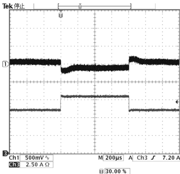
Fig-6: Output voltage response to load current step-change (6A-8A-6A) at Vin=48V. Top trace: Output voltage (500mV/div). Bottom trace: load current (2.5A/div). Current slew rate: 5A/us. Co=47uF ceramic and electrolytic capacitor 220uF . Time scale: 200us/div
