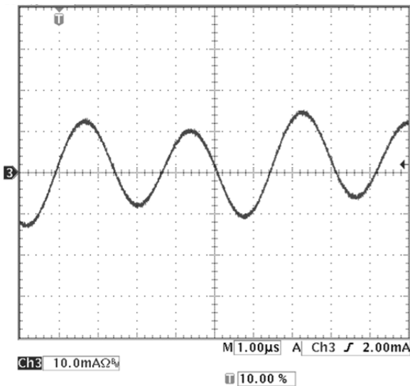
Fig-9: Input reflected ripple current, I_s (10mA/div), measured through 10uH at the source at full rated load current and V_{in}=48V . Time scale: 1us/div.
