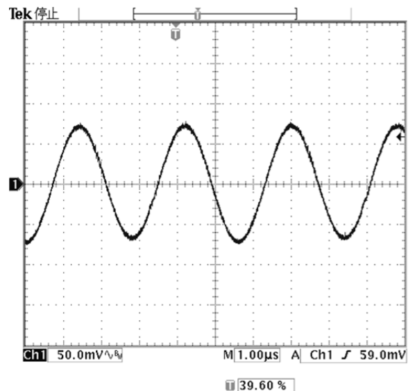
Fig-7: Output voltage ripple (50mV/div) at full rated load current into a resistive load with Co=220uF electrolytic capacitor and 47uF ceramic and Vin=48V. Time scale: 1us/div
