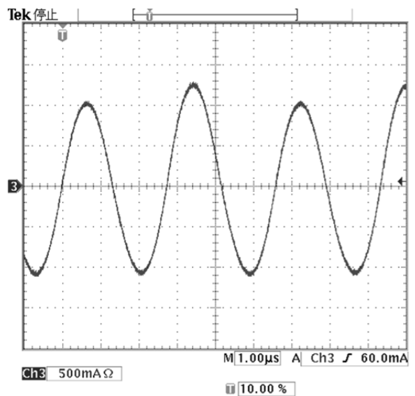
Fig-10: Input reflected ripple current, I_c (500mA/div), measured through 10uH at the source at full rated load current and V_{in}=48V . Time scale: 1us/div.
