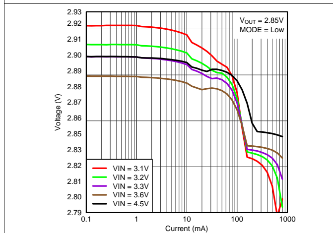
Figure 19. TPS82693 DC Output Voltage vs Load Current
