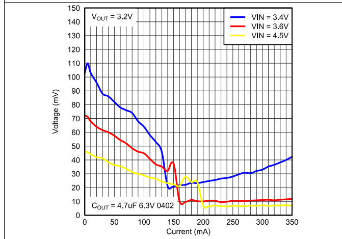
Figure 17. TPS82699 Peak-To-Peak Output Ripple Voltage vs Load Current
