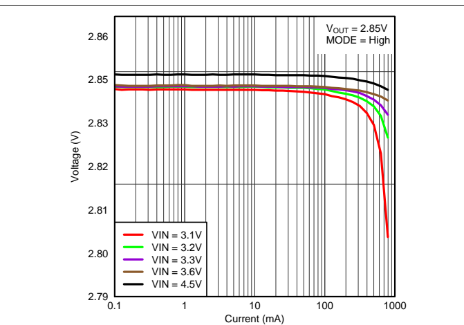
Figure 20. TPS82693dc Output Voltage vs Load Current
