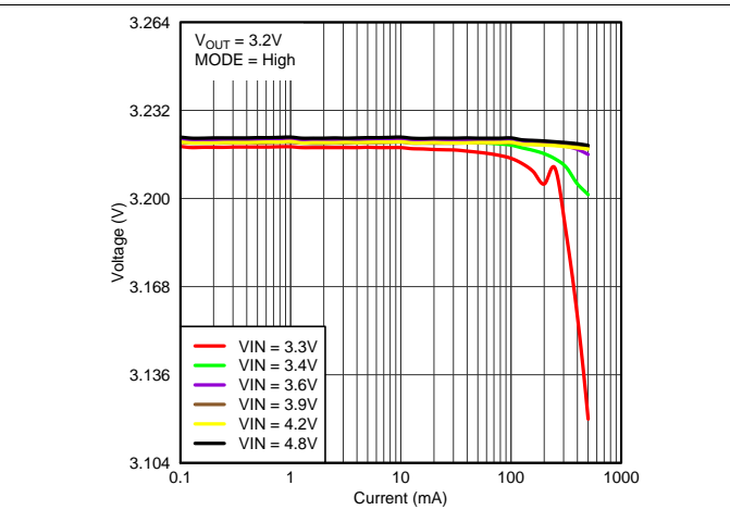
Figure 18. TPS82699 DC Output Voltage vs Load Current
