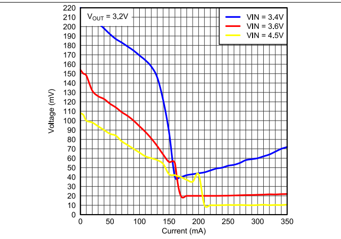
Figure 16. TPS82699 Peak-To-Peak Output Ripple Voltage vs Load Current
