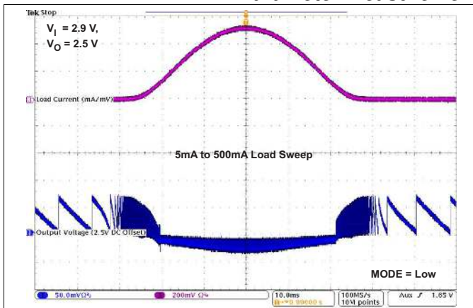
Figure 38. TPS826951 AC Load Transient Response
