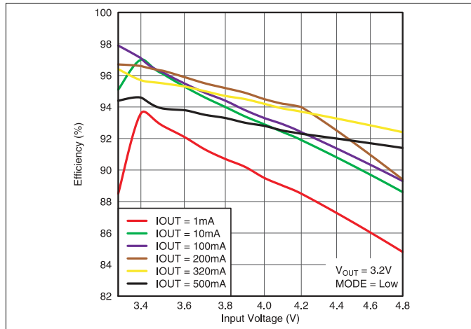
Figure 15. TPS82699 Efficiency vs Input Voltage
