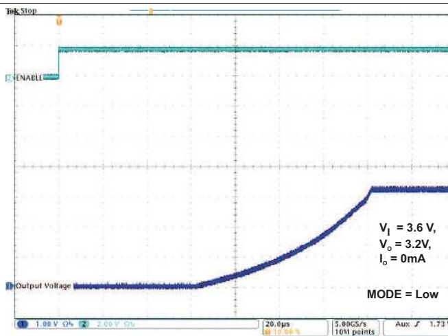
Figure 24. TPS82699 Start-Up
