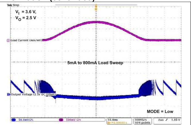
Figure 39. TPS826951 AC Load Transient Response
