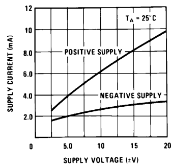
Figure 10. Supply Current
