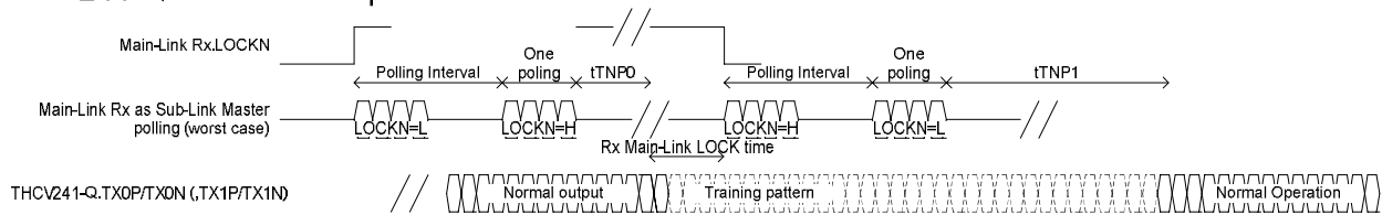
Figure 23. Re-Lock Sequence
