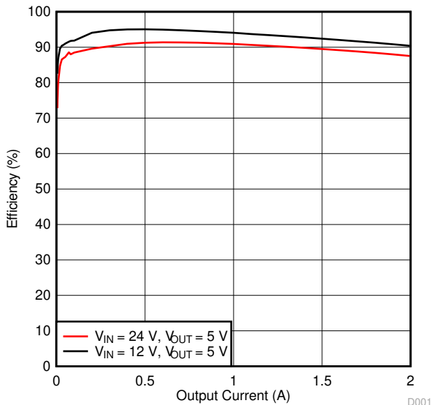
Figure 2-1. TPS54202HEVM-716 Efficiency
