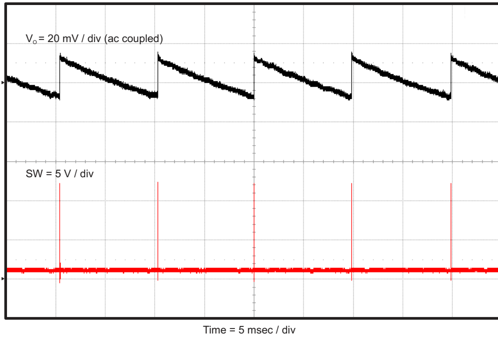
Figure 4-9. TPS563210EVM-663 Output Voltage Ripple, I_{OUT} = 0 mA
