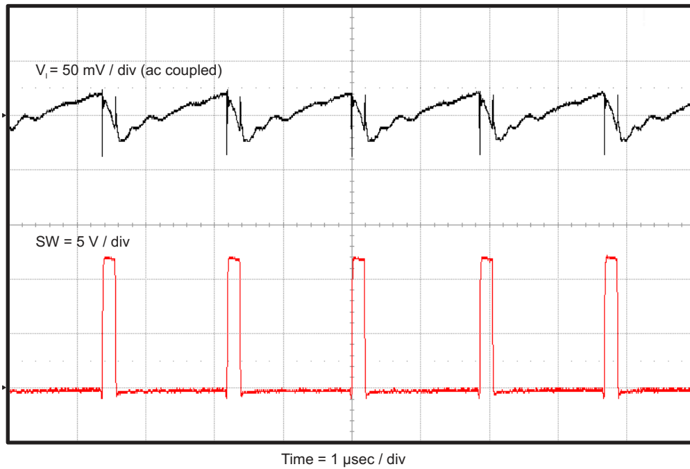
Figure 4-10. TPS563210EVM-663 Input Voltage Ripple, I_{OUT} = 3 A
