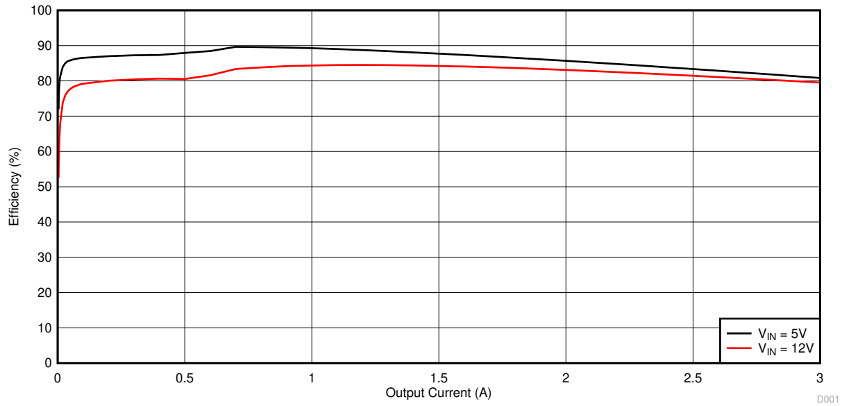
Figure 4-1. TPS563210EVM-663 Efficiency
