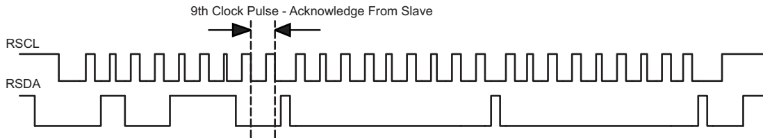
Figure 31. Bus-R Waveform
