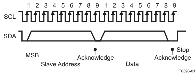
Figure 39. I 2 C Address, Data Cycle(s), and Stop
