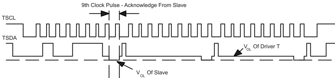
Figure 32. Bus T Waveform
