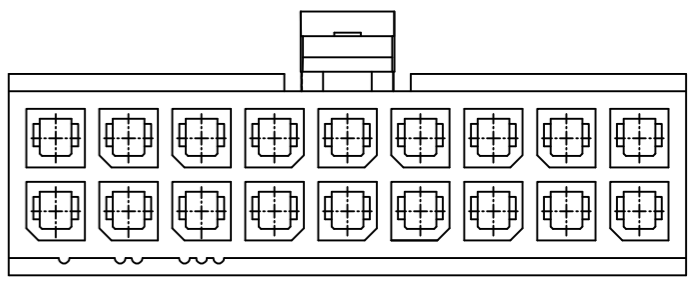
18 POS
