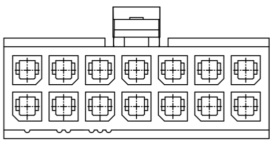
14 POS
