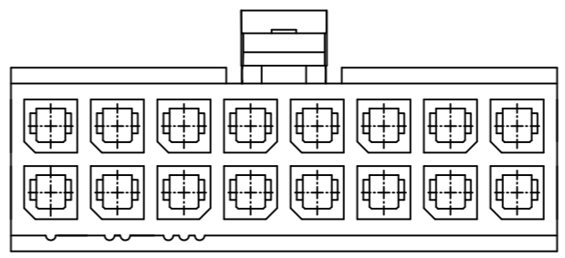
16 POS
