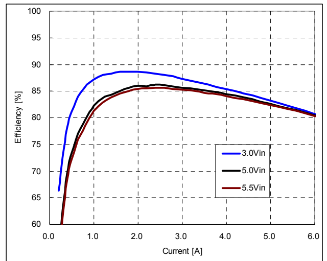
Fig.7: Efficiency vs. load current and input voltage for 1.2Vout
