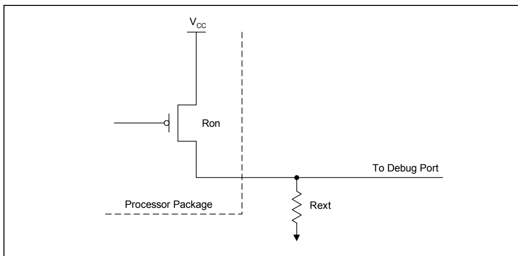
Figure 2-6. ITPCLKOUT[1:0] Output Buffer Diagram
