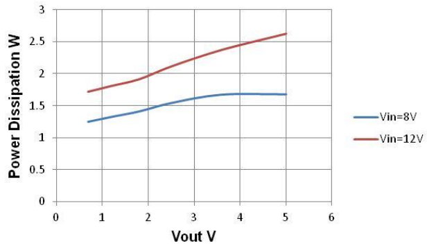
Figure 10. Power Dissipation vs Vout, Iout=5A, Fsw=1MHz
