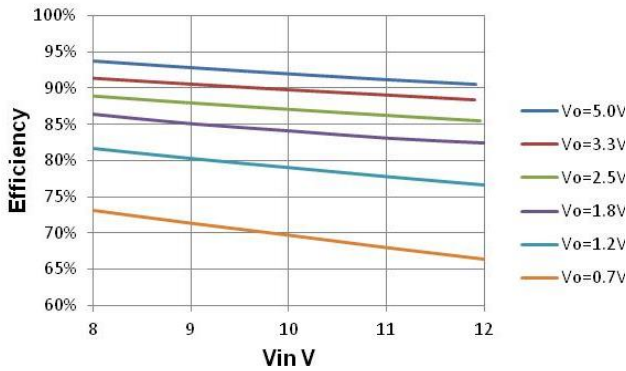
Figure 5. Efficiency vs Input Voltage at I_{out}=5A , F_{sw}=500kHz
