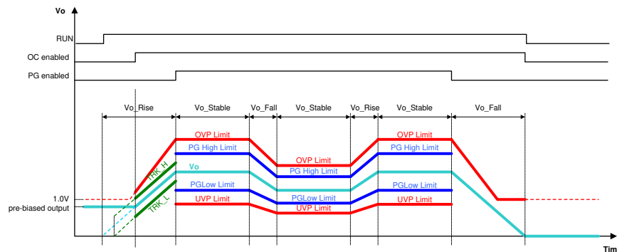
Figure 30. Protection Enable Conditions
