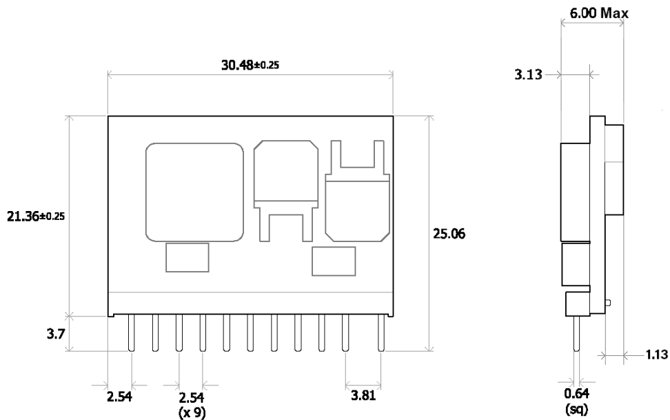
Figure 57. Recommended Footprint – Top View
