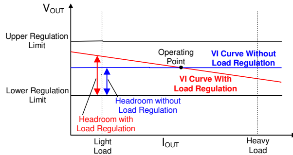
Figure 13. Optimal Voltage Positioning Concept
