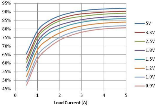
Figure 4. Efficiency vs. Output Voltage, I_{out}=5A , F_{sw}=500kHz
