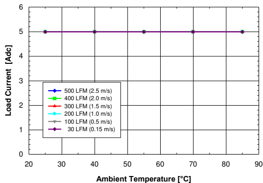
Figure 1. Available output current vs. ambient air temperature and airflow rates for converter DP8105G mounted horizontally with air flowing from input to output, MOSFET temperature \leq 120 °C, V_{in} = 12 V, V_{out} = 5 V, and F_{sw} = 500 KHz
