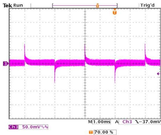
Figure 48. Transient Response with Regulation set to 0.0 mV/A.
