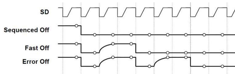
Figure 40. OK Severity Encoding Waveforms
